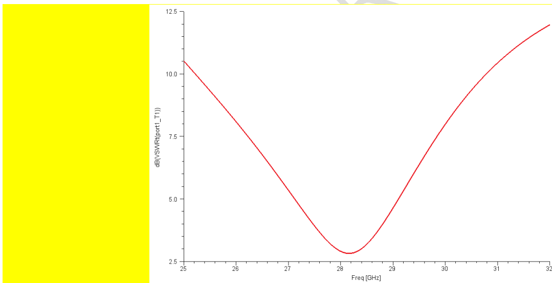
Fig. 14: VSWR of GA-optimized mm-wave antenna at 28 GHz
