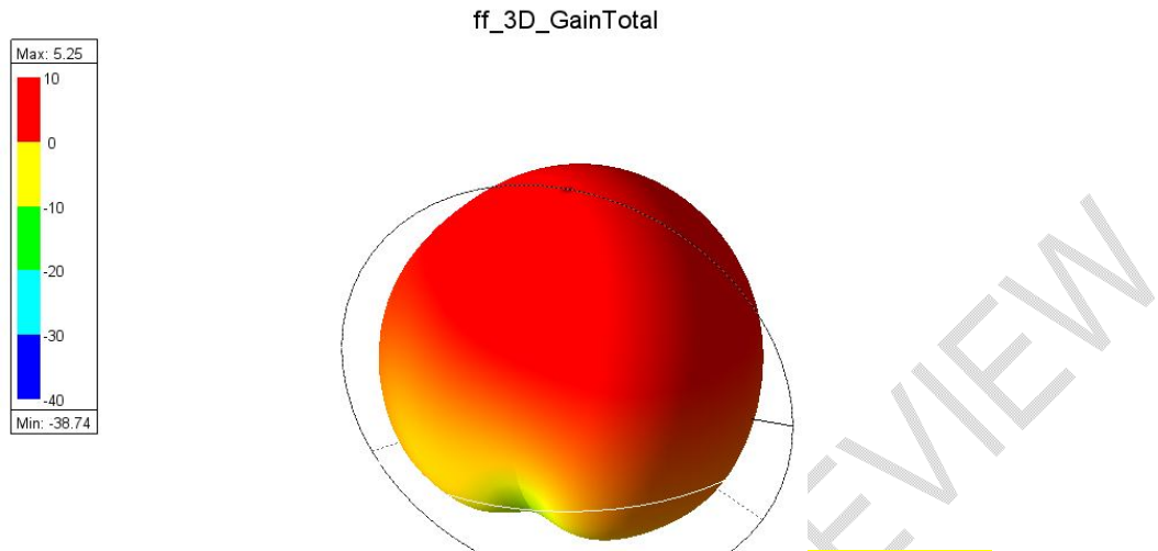
Fig. 9: Gain of unoptimized QWT-fed mmWave patch antenna at 28 GHz
