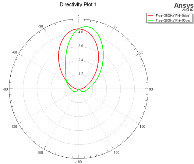
Fig. 11: E- and H-plane of the unoptimizedmmWave antenna
