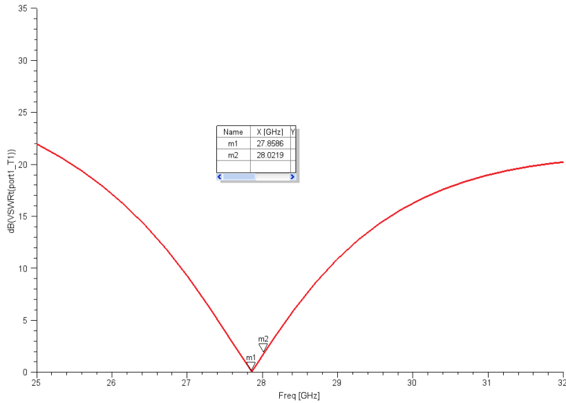
Fig. 13: VSWR of unoptimized mm-wave antenna at 28 GHz
