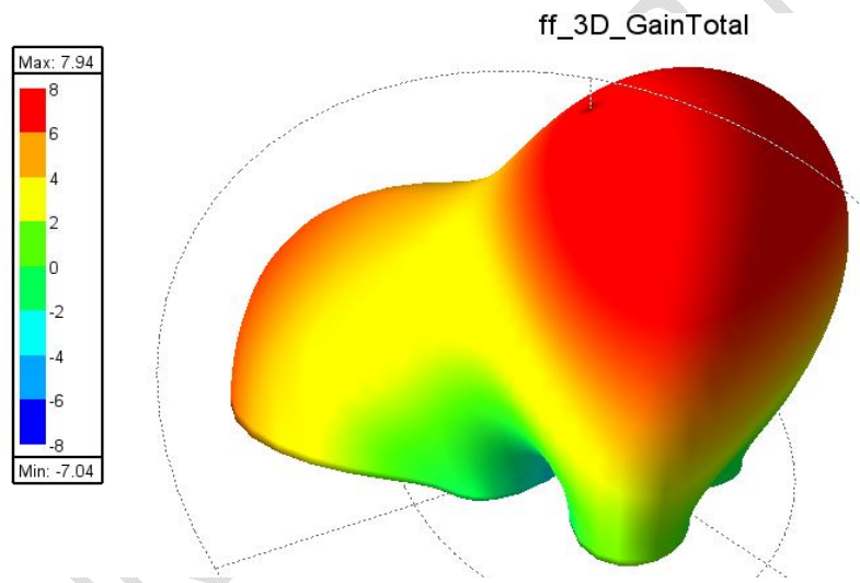
Fig. 10: Gain of GA-optimized QWT-fed mmWave patch antenna at 28 GHz
