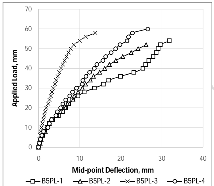
(b) Deflection of Beams Reinforced with B5PL Bars.
