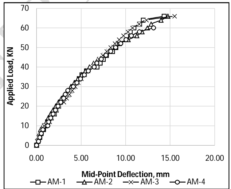
(d) Deflection of Beams Reinforced with AM bars.
