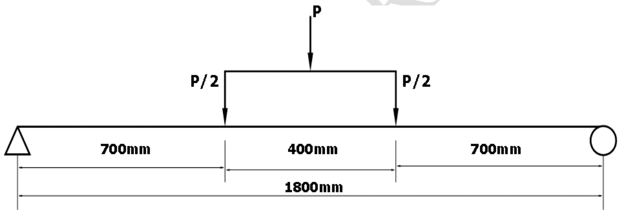
Fig.4: Diagrammatic representation of loaded beam specimen
