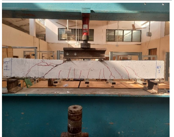
Fig 3: Beam Specimens during and after testing.
