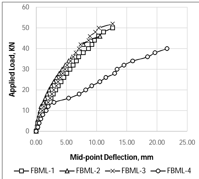
(c) Deflection of Beams Reinforced with FBML bars.
