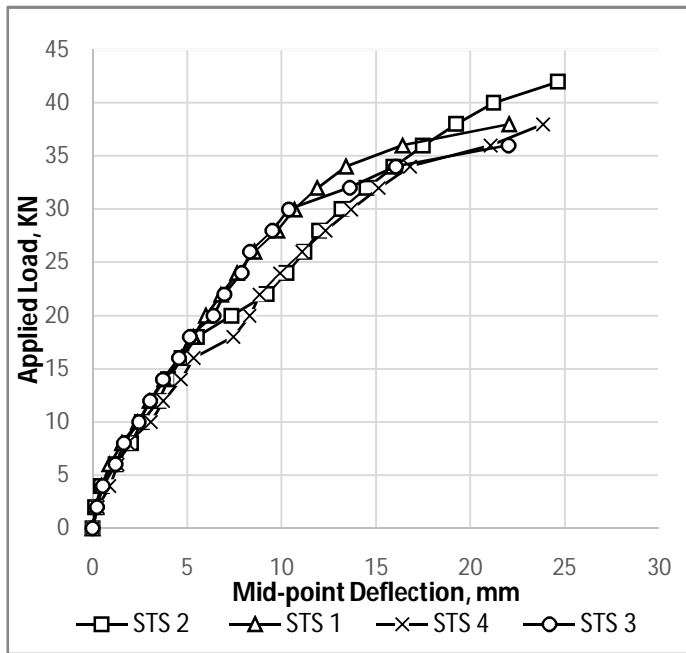
(a) Deflection of Beams Reinforced with STS Bars.
