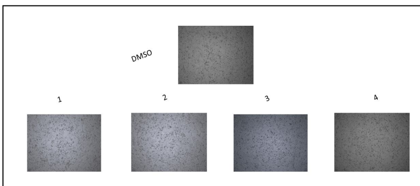
Figure 1: The Phase contrast image shows specific and significant morphological change. The serial 1,2,3,4 refers the concentration of MECC from 125 to 1000 \mu\text{m/L} as shown in table 2.
