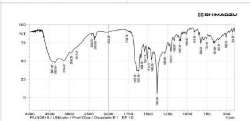
Fig 3. IR Spectra of the Ligand and Metal complexes
