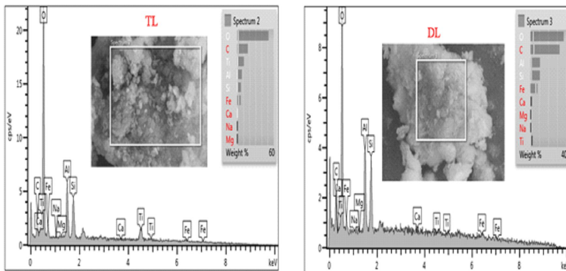
Fig. 6. EDX spectra of the TL and DL on a 2.5 \mu\text{m} scale SEM image
