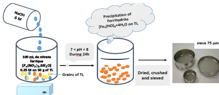
Fig. 1. Protocol for the preparation of DL laterite
