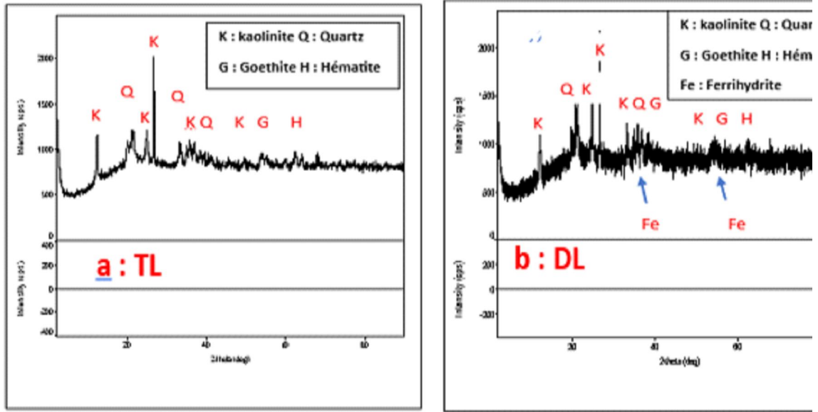
Fig. 4. Diffractogram of the mineral phases of TL and DL
