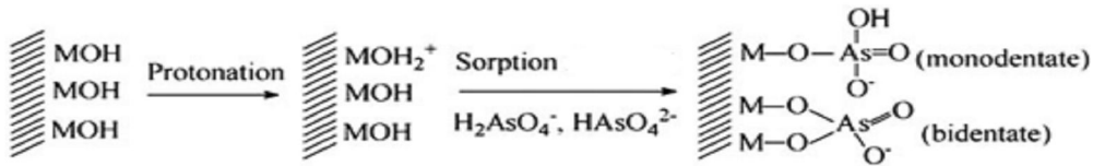
(a) Surface complex for As(V) sorption With -M = TL or DL adsorbent
