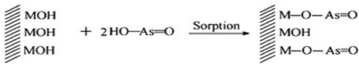
(b) Surface complex for As(III) sorption
