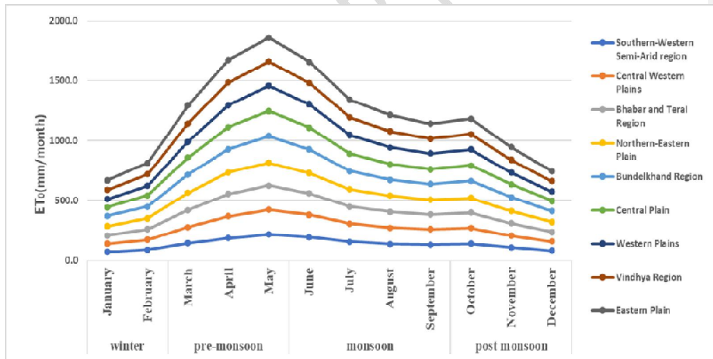
Figure 1 Reference Evapotranspiration
