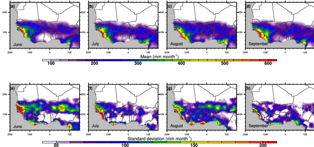
Fig. 3. Rainy months mean and standard deviations of rainfall over West Africa (1960-2022)
