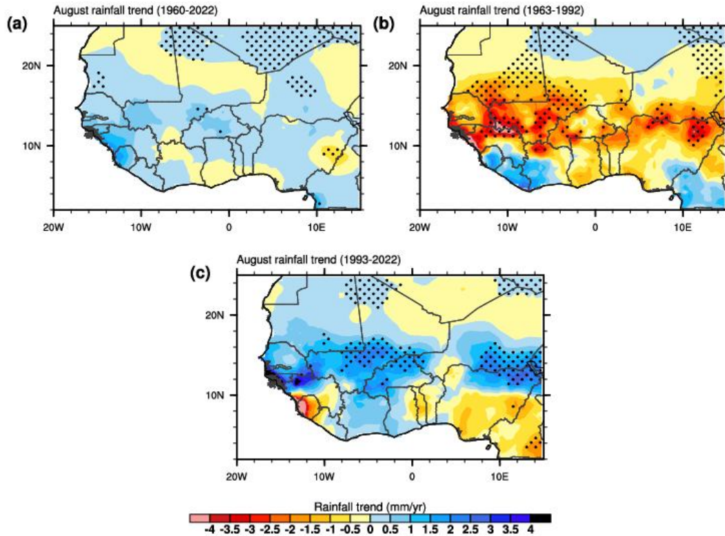
Fig. 7. Patterns of August rainfall trend over West Africa for a) 1960-2022, b) 1963-1992, and c) 1993-2022
