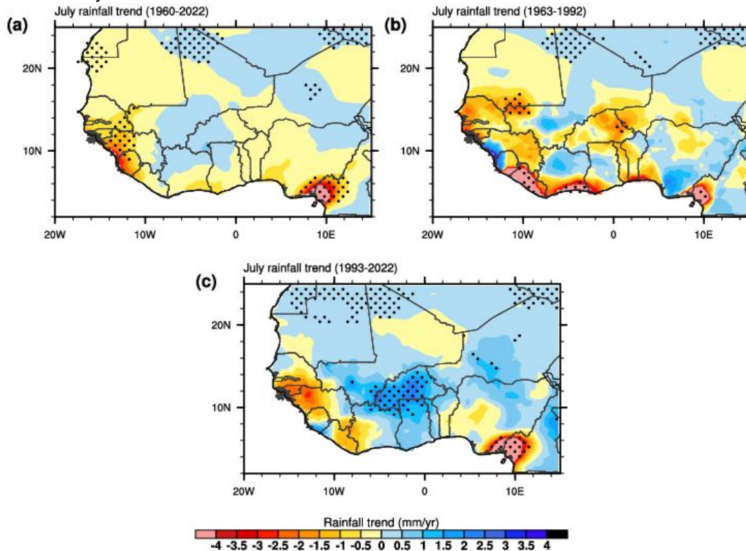
Fig. 6. Patterns of July rainfall trend over West Africa for a) 1960-2022, b) 1963-1992, and c) 1993-2022
