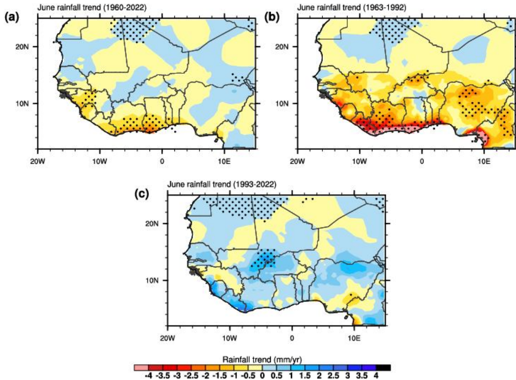
Fig. 5. Patterns of June rainfall trend over West Africa for a) 1960-2022, b) 1963-1992, and c) 1993-2022
