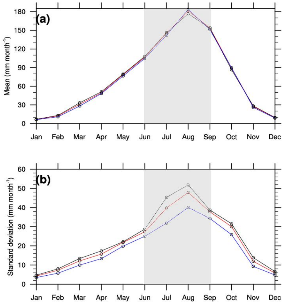
Fig. 2. Seasonal cycle of the (a) mean and (b) standard deviation of rainfall averaged over West Africa during the three study periods: Red (1960-2022), black (1963-1992) and Blue (1993-2022).
