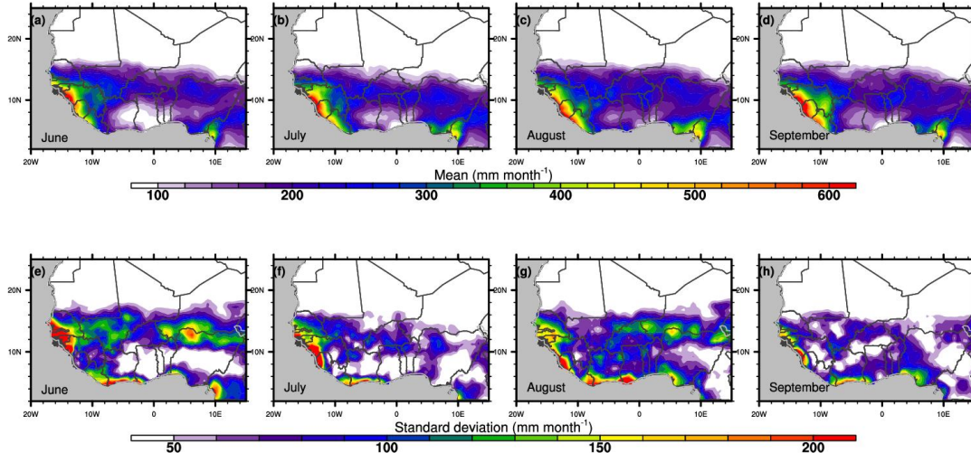
Fig. 3. Rainy months mean and standard deviations of rainfall over West Africa (1960-2022) The absence of notable differences in the seasonal cycle of mean rainfall during the three periods buttresses the idea that the seasonal rainfall cycle has remained relatively the same during the three periods. This may be due to variability in intraseasonal rainfall properties such as frequencies, intensity and duration [38,39]. The observed variability in the seasonal cycle (Figures 2b and 3b) shows notable temporal changes in the three periods, as months and areas of higher rainfall occurrence depict higher variability. June, July and September show a significant decline, while August rainfall trend has remained relatively stable over the entire period. Since the Sahel pattern of rainfall variability is the leading mode of West African rainfall, this result supports Nicholson [1], who states that anomalies in August and September significantly contribute to the enhanced inter-annual variability in Sahel rainfall. A similar result was reported by [40] for Togo.
