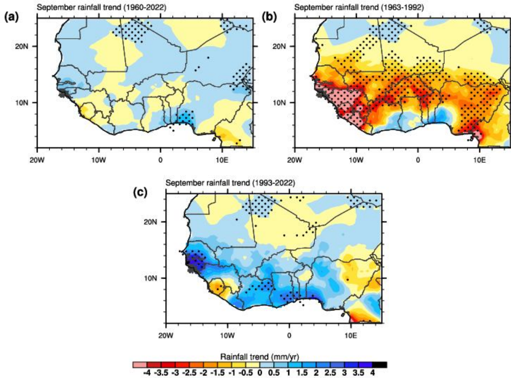
Fig. 8. Patterns of September rainfall trend over West Africa for a) 1960-2022, b) 1963-1992, and c) 1993-2022
