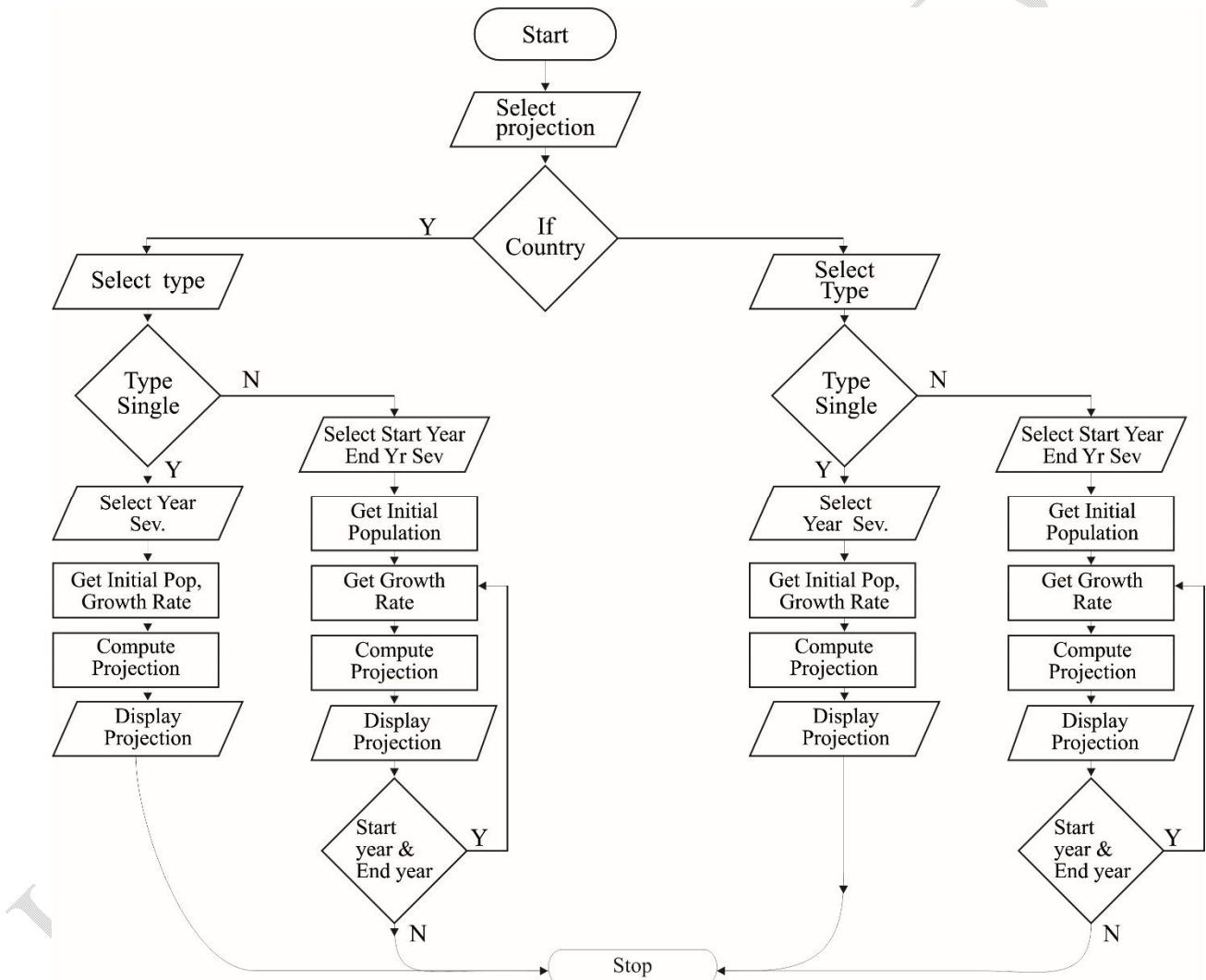
Figure 2: Flow chart showing the logic that the machine use to learn the logic to carry out the sequential method of the projection of 2006 conducted population census.
