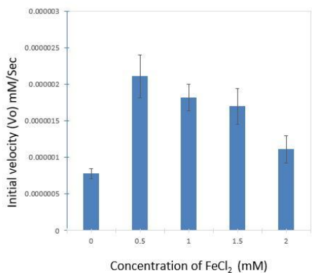
Figure 2: Effect of FeCl_2 concentrations on the peroxidase activity in watermelon peel
