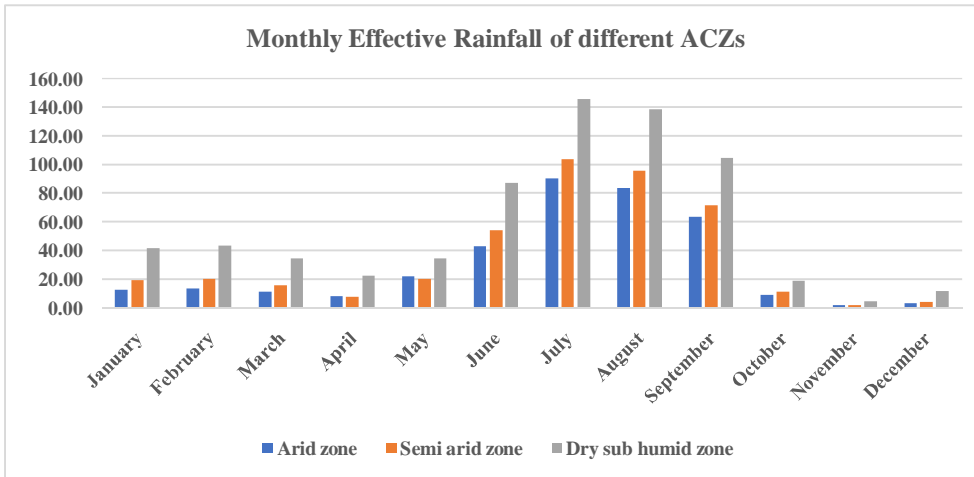
Figure 2 Effective Rainfall
