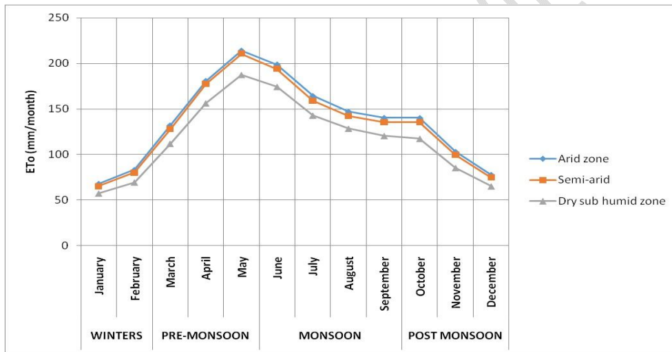
Figure 1 Reference Evapotranspiration
