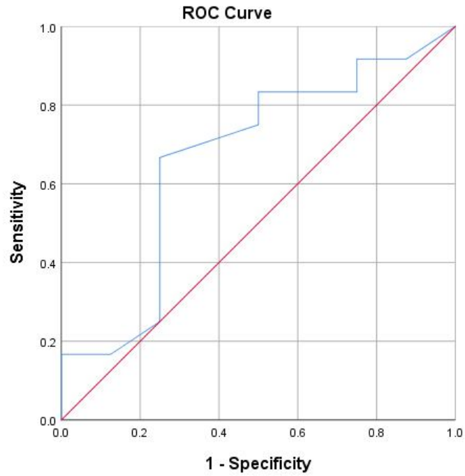
Figure (5): ROC (Receiving operating curve) for RI's diagnostic performance to discriminate malignant from benign lesions.
