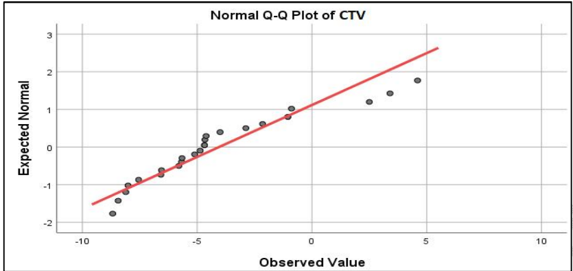
Figure 12: Normal Q-Q plot of CTV distribution.
