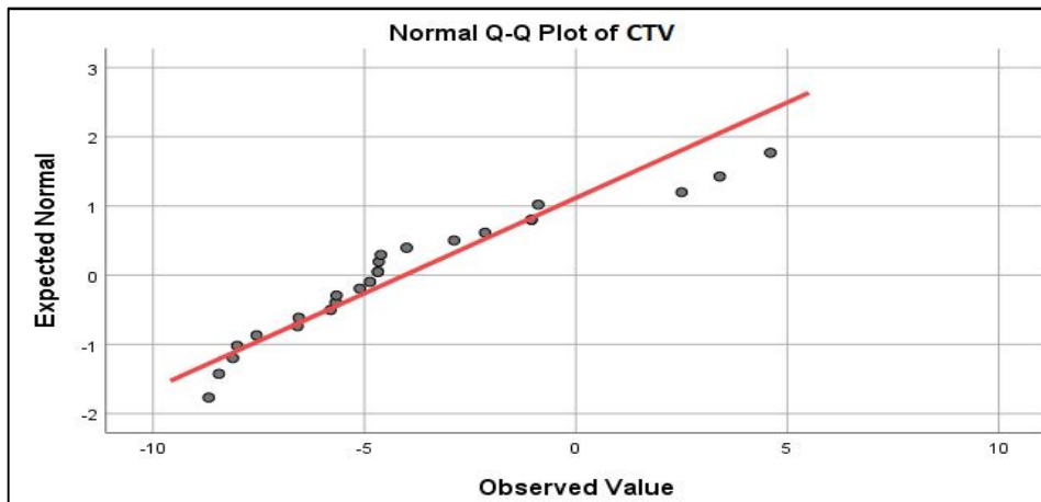
Figure 12: Normal Q-Q plot of CTV distribution.
