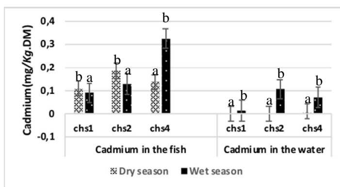
Figure 3. Variation of Cadmium water and fish meat concentrations in samples during the dry (a) and the wet season (b).
