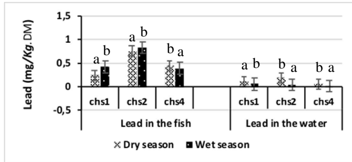
Figure 2. Variation of lead water and fish meat concentrations in samples during the dry (a) and the wet season (b).
