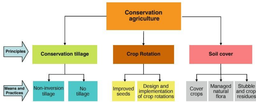
Fig. 1: The three principles of conservation agriculture and the main practices and means needed to achieve each principle [33]
