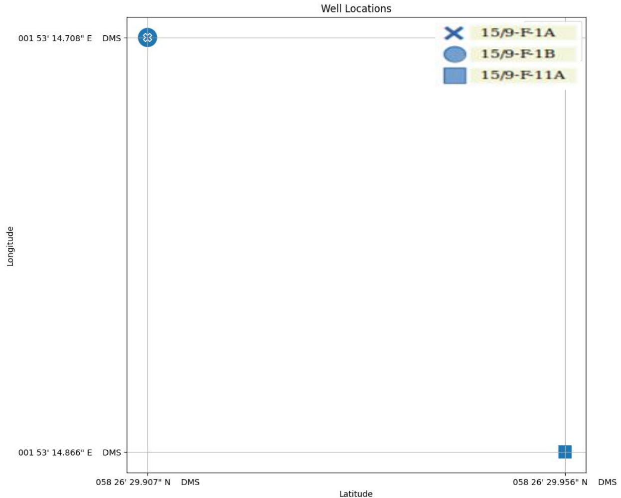
Fig. 3. Plot showing well locations.
