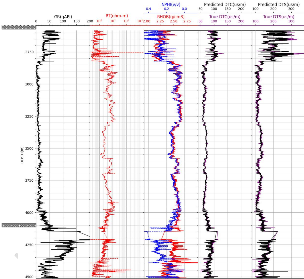
Fig. 8 Plot showing the predicted and measured DTC and DTS in 15/9-F11T2, along with the identified seal formations (in red and blue).
