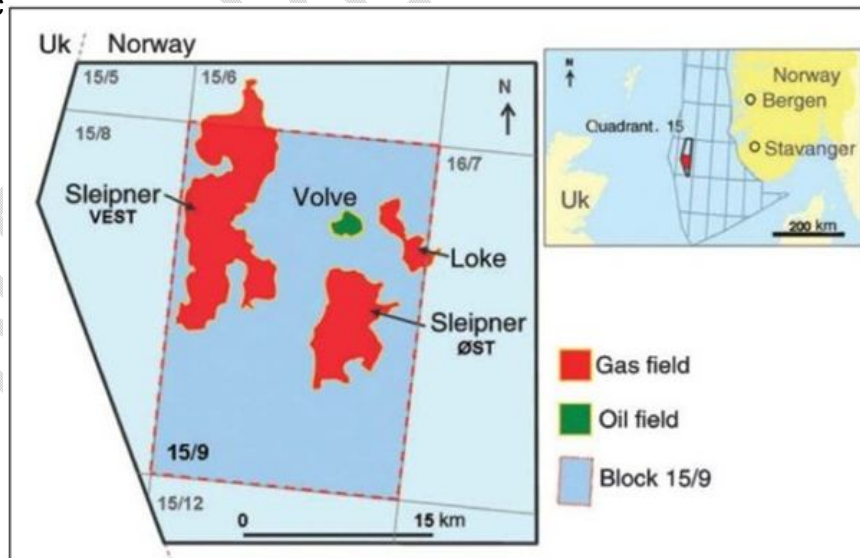
Fig. 1. Location of Volve within the Block 15/9
