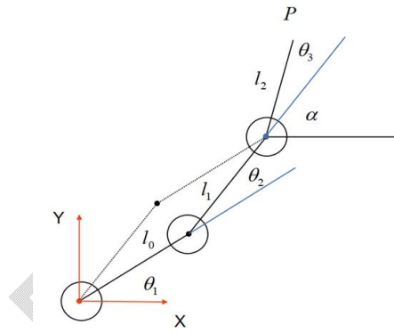
Fig. 4 Mechanical arm movement diagram
