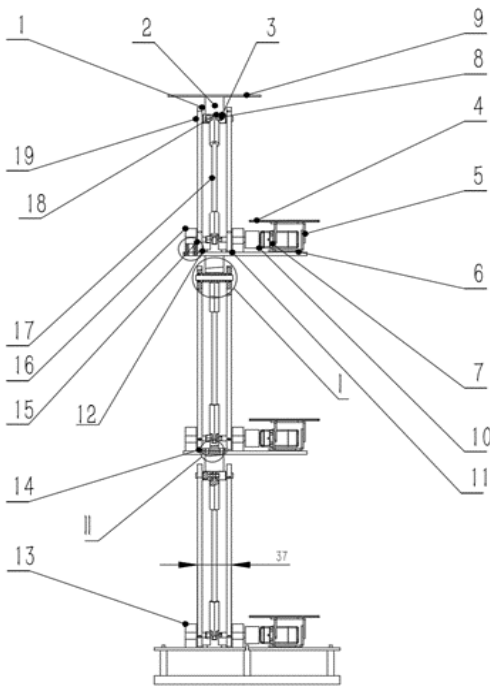
Fig. 1 Structural design of robotic arm
