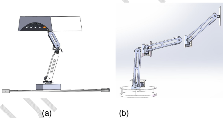
Fig.11 Mechanical arm demonstrates
