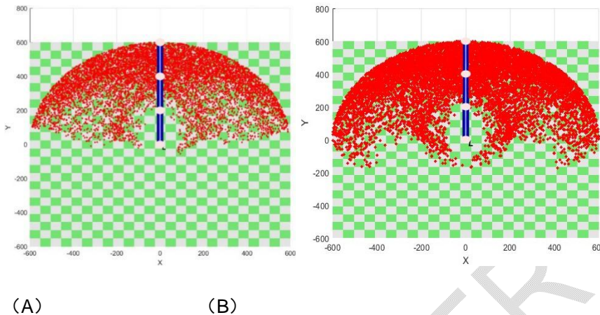
Fig. 7 Robotic arm workspace set
