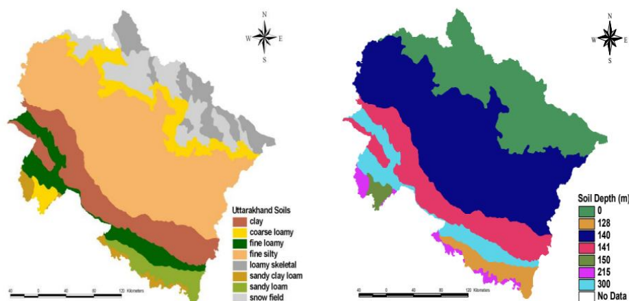
Fig. 2 .Uttarakhand soils and soil depth mapping by NBSS&LUP
