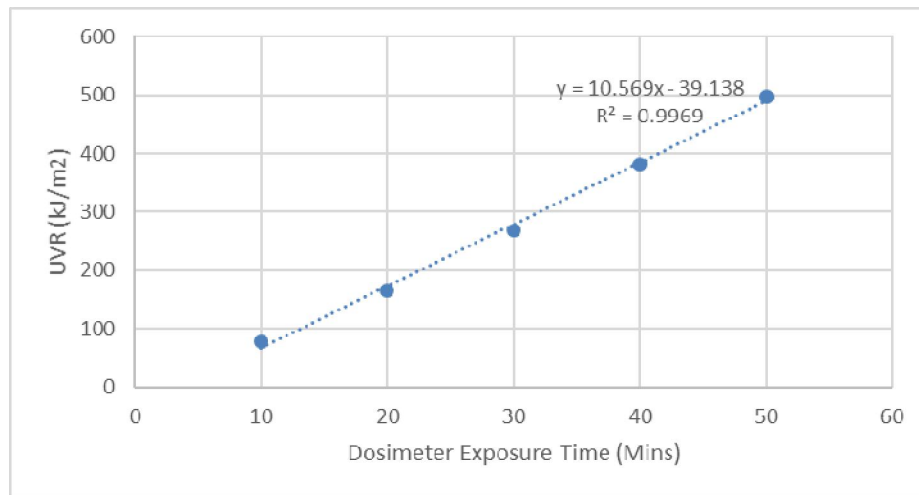
Fig. 5. Dosimeter calibration curve at river bank (Wadata Axis)
