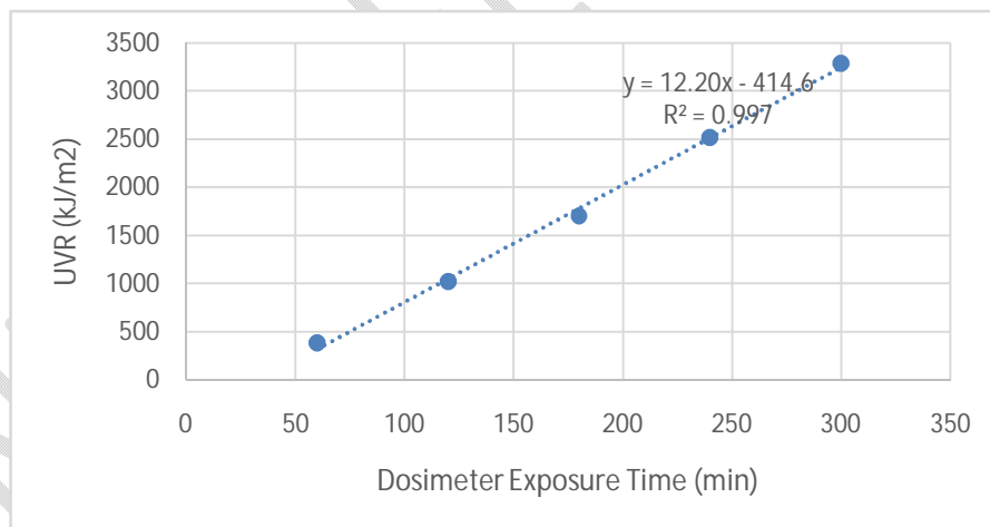
Fig. 3. Dosimeter calibration curve at Wurukum Market
