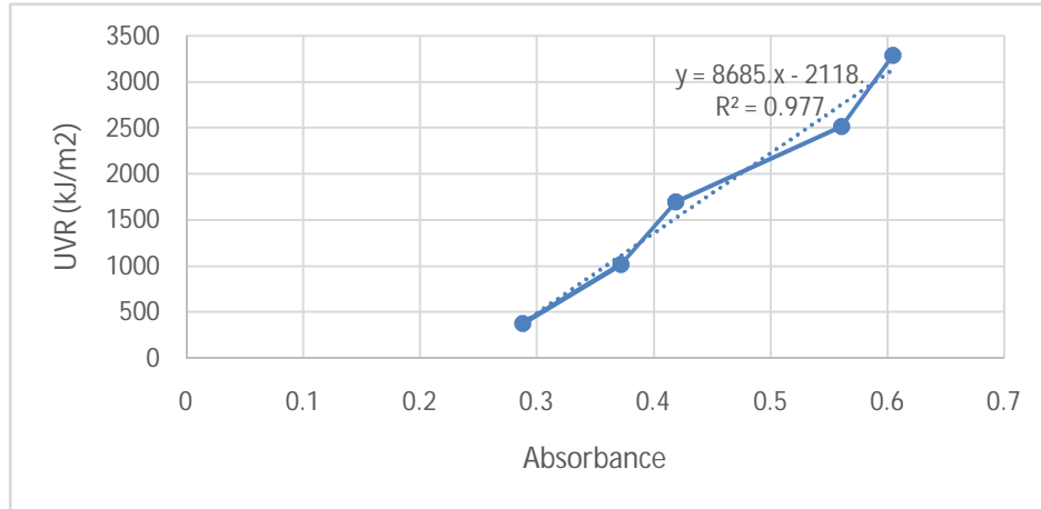
Fig. 4. Dosimeter response curve at Wurukum Market
