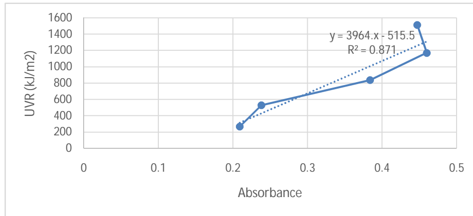
Fig. 8. Dosimeter response curve at Benue State University
