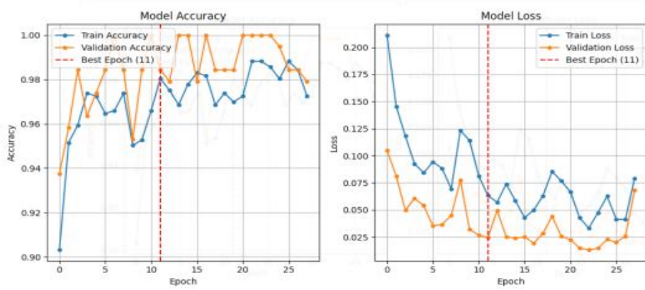
Figure 4: ANN Training Process
