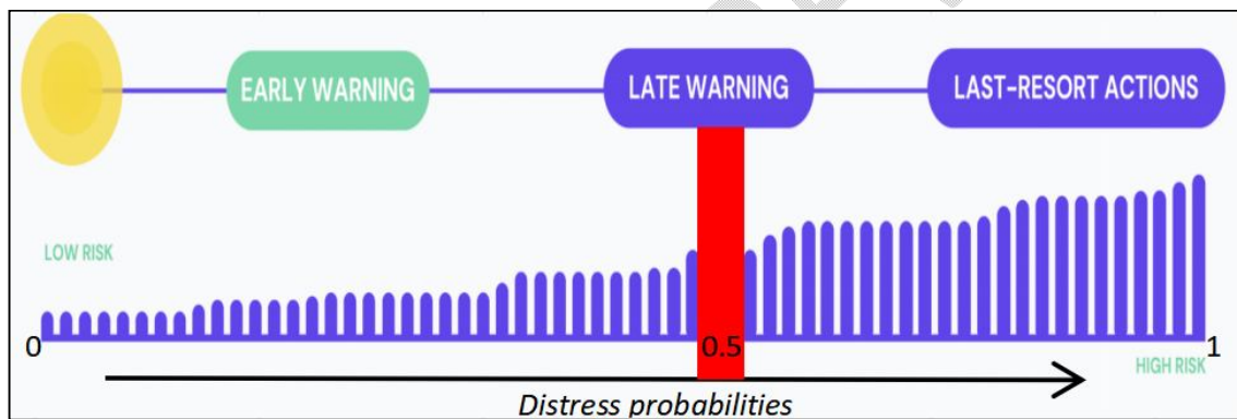
Figure 2: EWS Model
