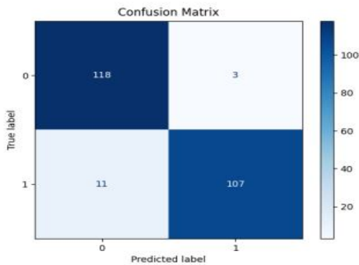
Figure 5: Confusion Matrix
