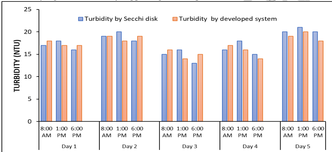
Fig.6: Comparison of turbidity value with both methods
