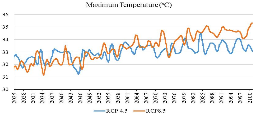
Fig 2: Trend of maximum temperature (°C) under RCP 4.5 and RCP 8.5 scenarios during projection period (2025-2100).
