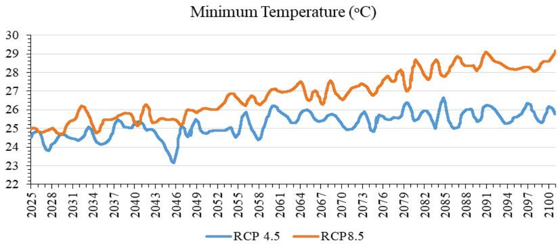
Fig 1: Trend of minimum temperature (°C) under RCP 4.5 and RCP 8.5 scenarios during projection period (2025-2100).
