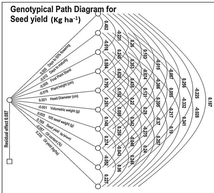
Fig. 4. Genotypic path diagram for seed yield ( \text{kg ha}^{-1} )
