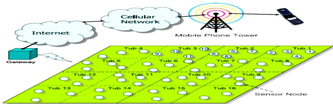
Fig. 2 Wireless sensor network [35]
