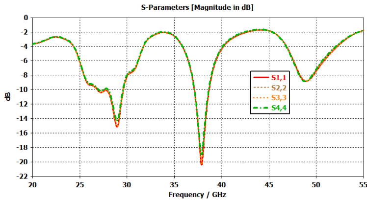
(a) Reflection coefficients
