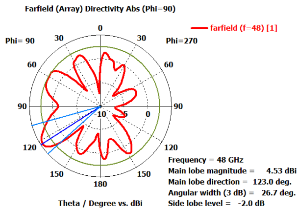
Fig. 8 Radiation patterns of 2 x 2 Minkowski fractal MIMO antenna with CRLH
