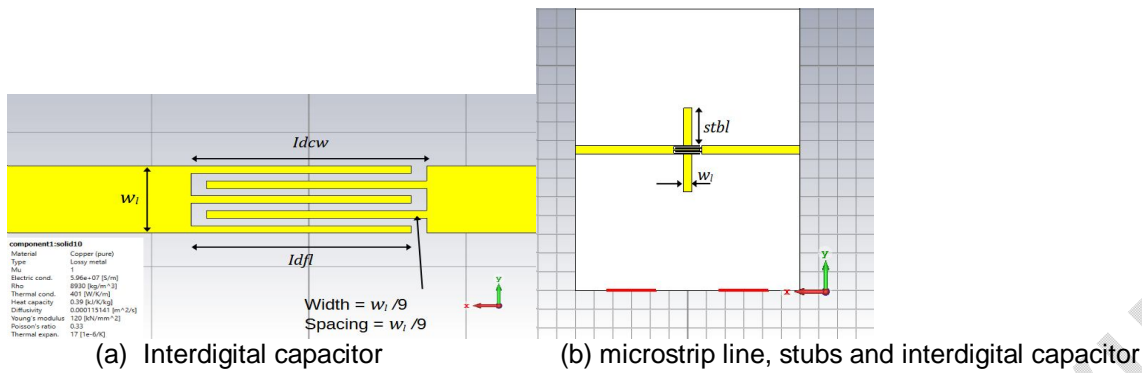
Fig3. CRLH structure
