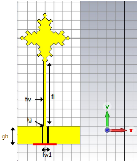
Fig. 2 Layout of second-order fractal antenna
