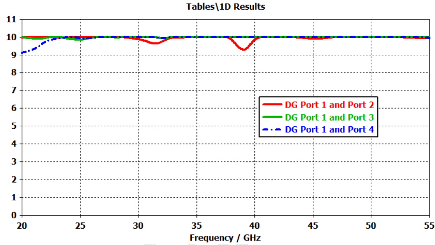
(b) Diversity Gain (DG) between antenna ports
