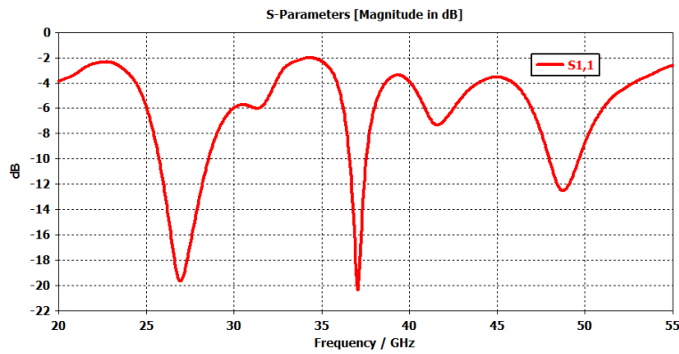
(a) Reflection coefficient
