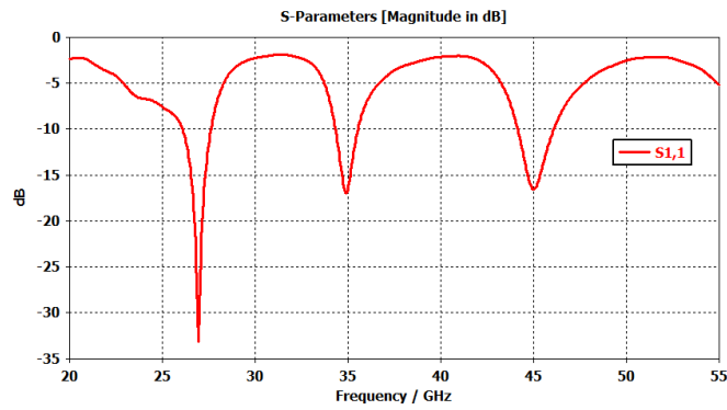
Fig. 5 Reflection coefficient of single second-order Minkowski fractal
