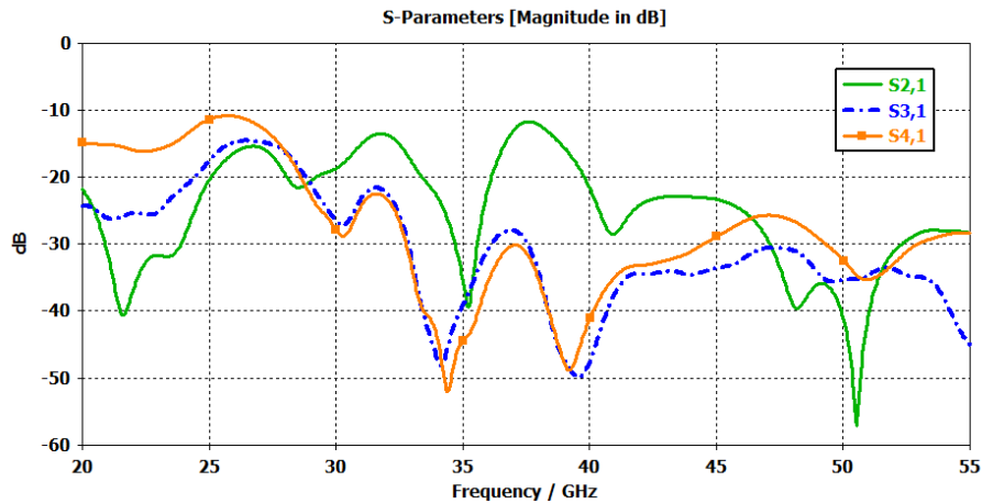
(a) Transmission coefficient
