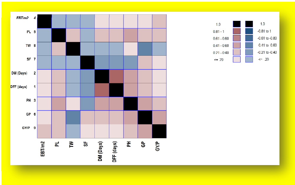
Figure .2 Phenotypic Correlation matrix for yield and yield component traits
