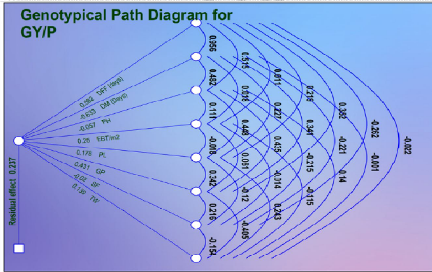
Figure .4 Genotypic path diagram for yield and its contributing traits
