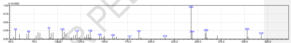
8-Piramen-18-oate <methyl->
