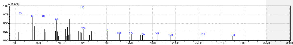
Manool <7-alpha-hydroxy->
