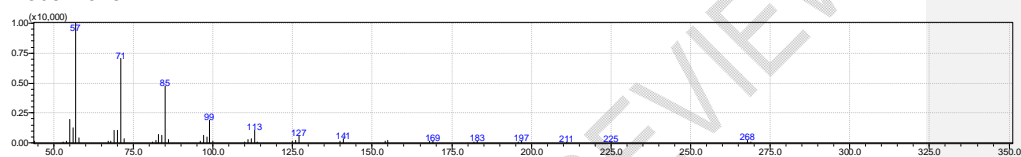
Nonadecane <n->
