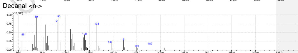
Caryophyllene <(E)>
