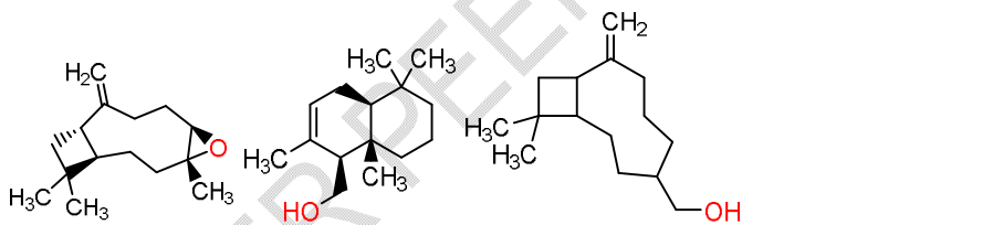
14-hydroxy-4,5-dihydro- Caryophyllene
