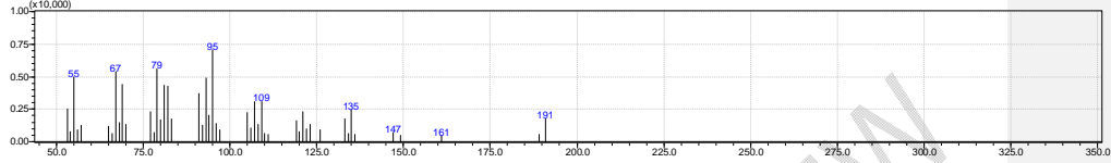
Caryophyllene <14-hydroxy-4,5-dihydro->
