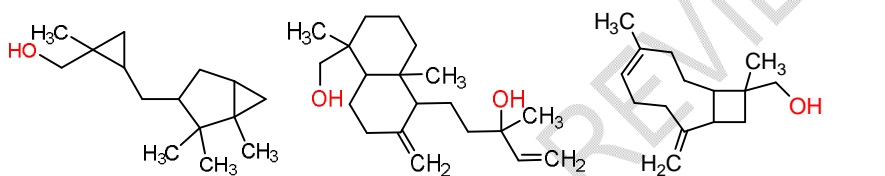
14-hydroxy-9-epi-(E)- caryophyllene
