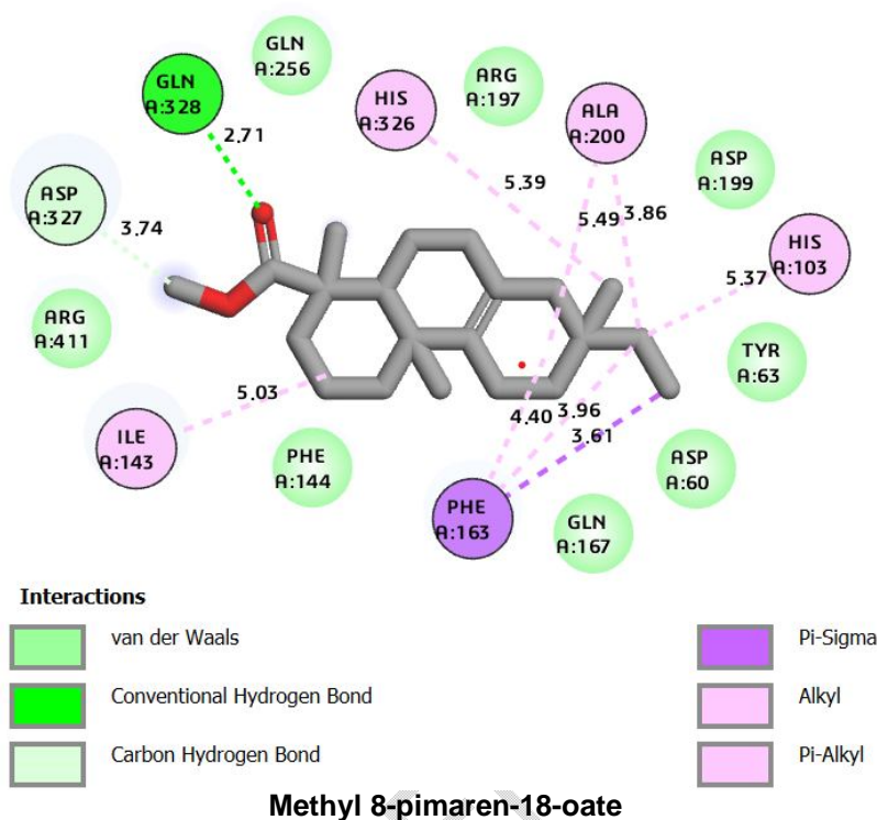
Fig. 2. 2D interactions of top three ligands with \alpha -glucosidase (PDB ID: 5ZCC)
