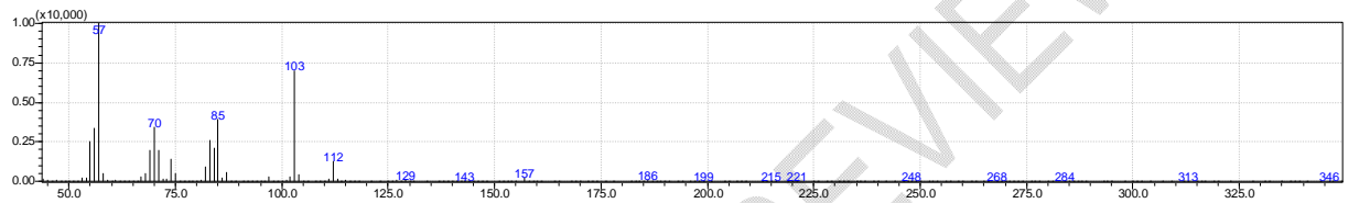
Butyrate <2-methyl-, octyl->
