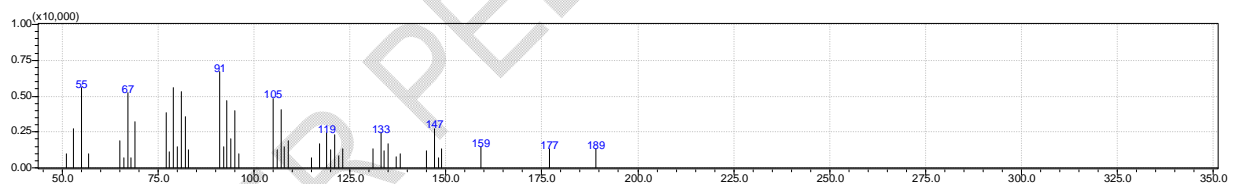
Aromandendrene epoxide <allo->
