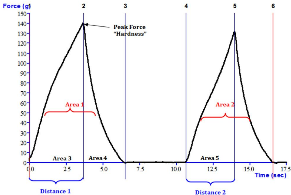
Fig. 1. Force –time (gram-sec)
