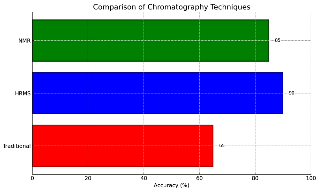
Figure 3: Comparison between traditional and advanced chromatography techniques in detecting urine sample manipulation (28).
