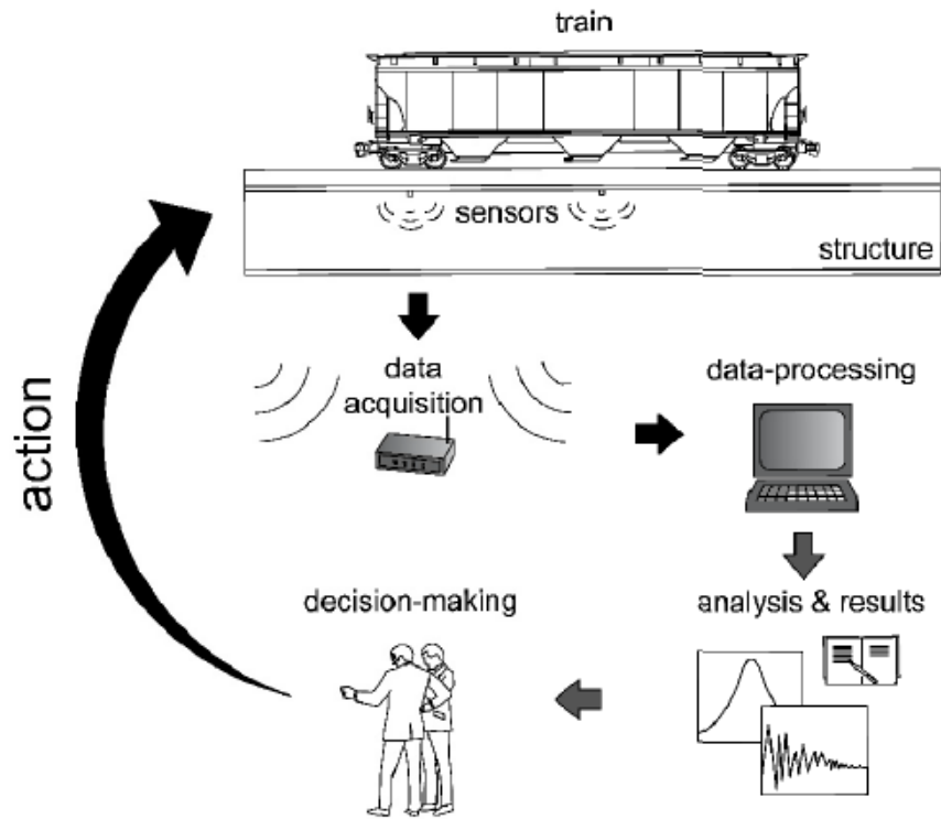
Figure 2: Schematic representation of the SHM of bridges
