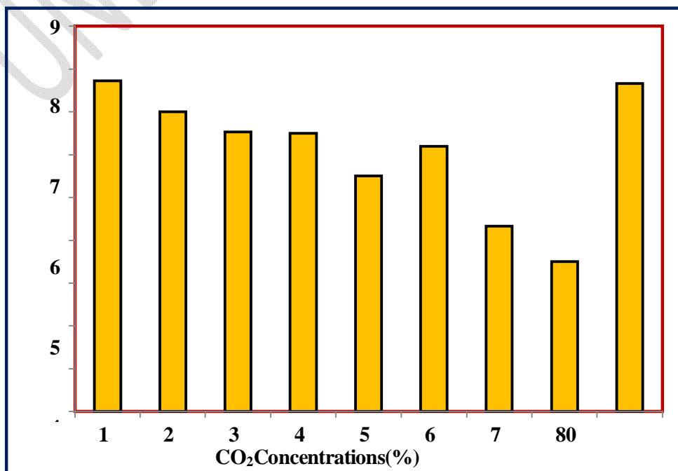
Figure 1. Effect of elevated levels of CO 2 on adult longevity (days) of pulse beetle C.
