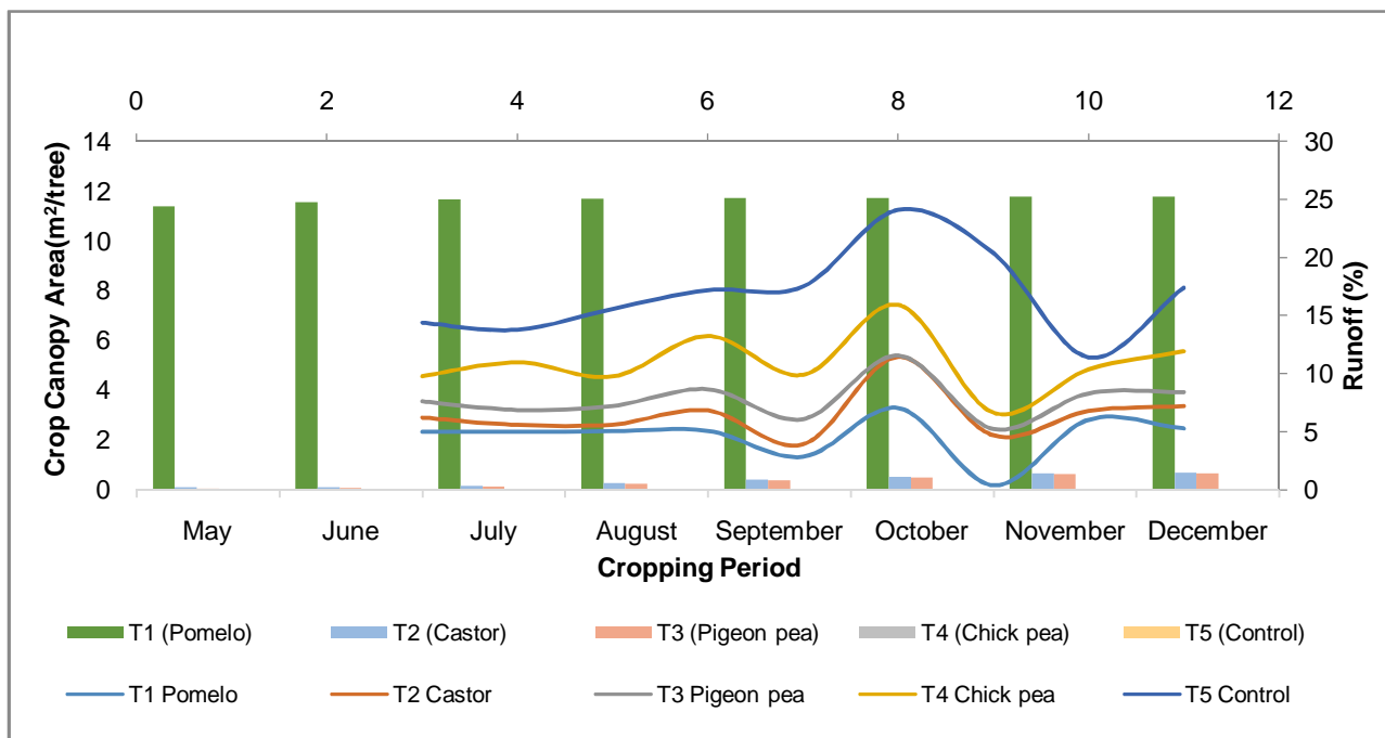
Fig.8. Runoff variations among the treatments during different stages of cropping period.
