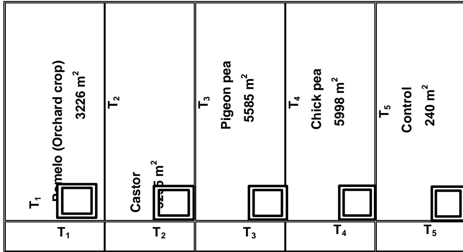
Fig. 3. Plan and layout of experimental site
