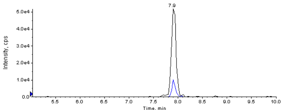
Fig. 1. Total ion chromatograph of azoxystrobin at 0.05 mg \text{kg}^{-1} in tomato fruits.
