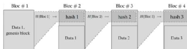
Figure2:Blockstructure[29]
