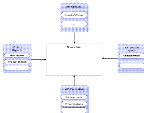
Figure4:Retrievingdatafromtheblockchain
