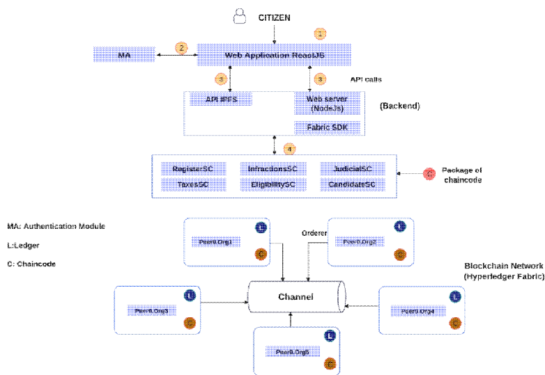
Figure 7: System operation
