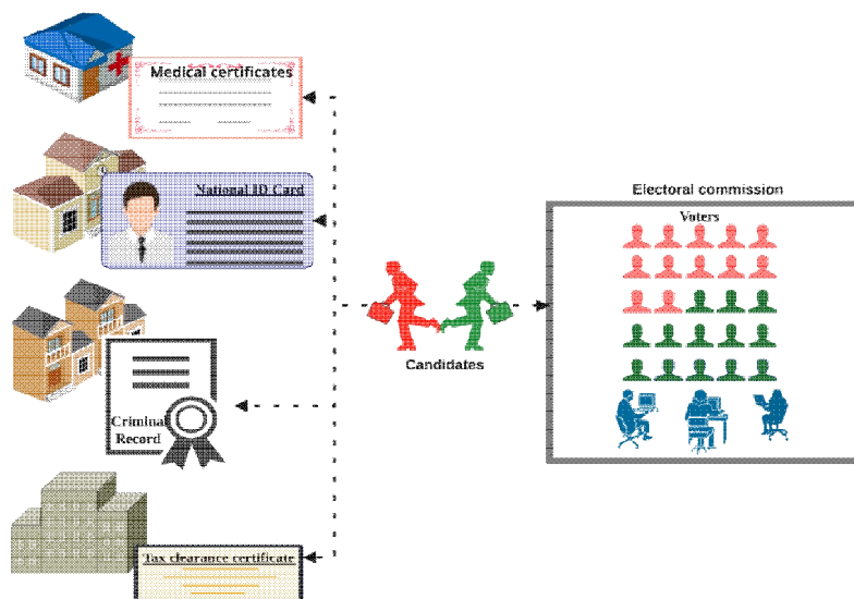
Figure3: Traditionaleligibilitycheckprocedure
