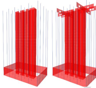
Figure .5 – (a) ETABS model for case 1; (b) ETABS model for case 2
