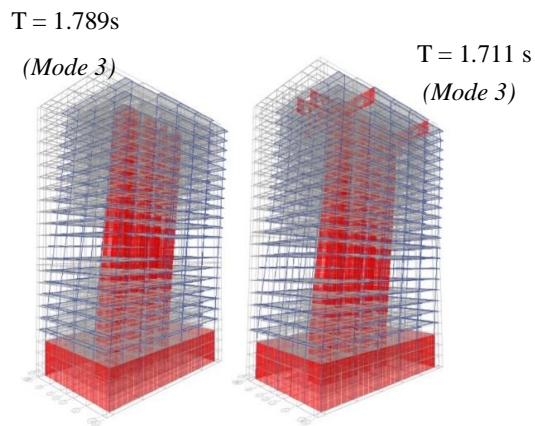
Figure 8 Mode Shape along X-direction for all Cases
