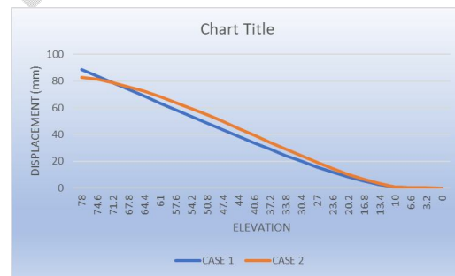
Figure 10 Total Displacement for All Cases along X and Y Directions
