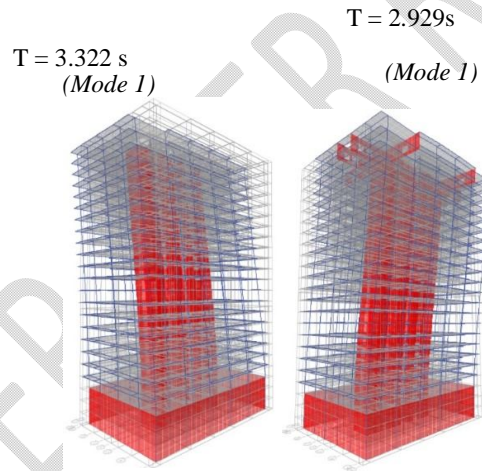
Figure 7 Mode Shape along Y-direction for all Cases
