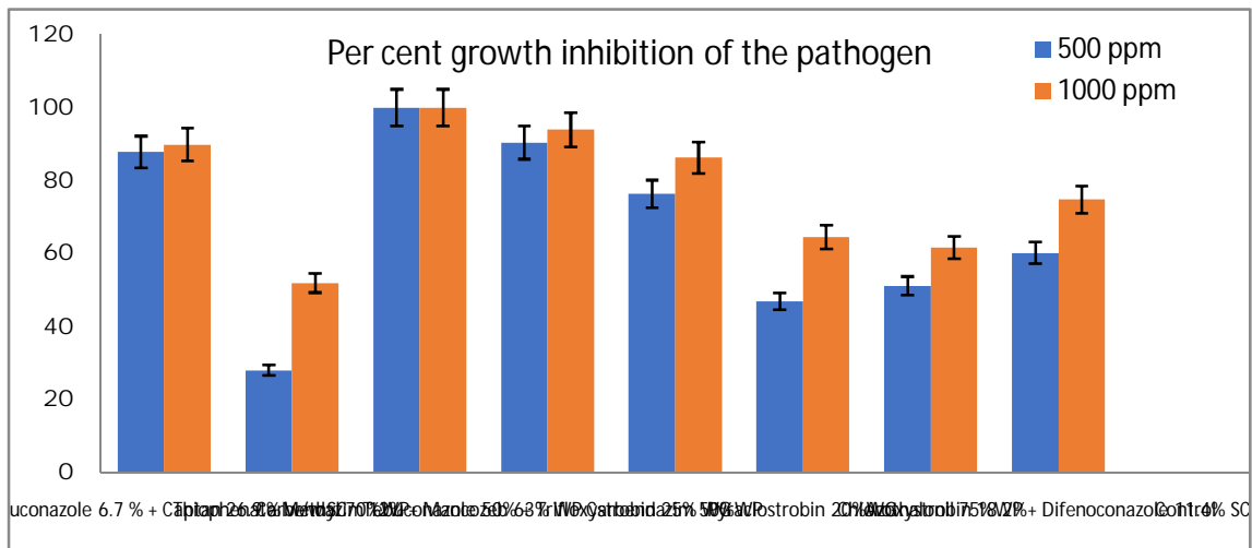
Fig. 1 Per cent growth inhibition of Fusarium oxysporum f. sp. capsici under in vitro conditions
