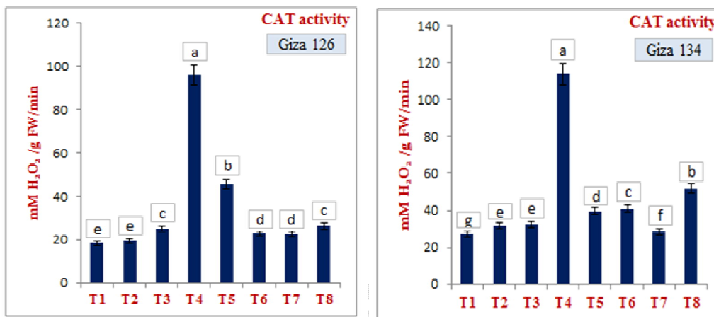
Figure (6): Effect of Salicylic Acid (SA) and Chitosan on Catalase (CAT) activity in barley leaves for the two studied genotypes, Giza 126 and Giza 134 under water stress conditions. T 1 =Control, T 2 =100ppm, T 3 =200ppm, T 4 =300ppm of salicylic acid, T 5 =150ppm, T 6 =225ppm, T 7 =300ppm of chitosan and T 8 =salicylic acid 100ppm and chitosan 150ppm mixture.
