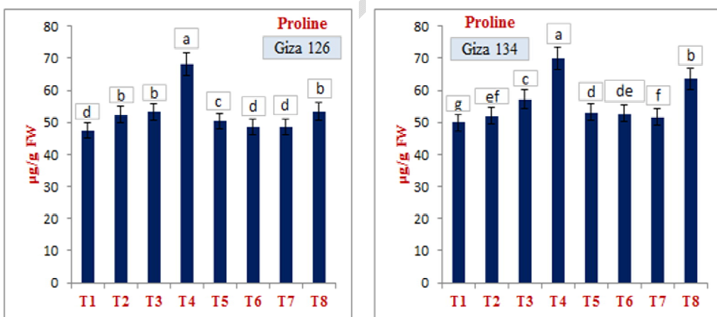
Figure (3): Effect of SA and Chitosan on accumulation of proline content in the two studied barley genotypes, Giza 126 and Giza 134 under water stress conditions. T 1 =Control, T 2 =100ppm, T 3 =200ppm, T 4 =300ppm of salicylic acid, T 5 =150ppm, T 6 =225ppm, T 7 =300ppm of chitosan and T 8 =salicylic acid 100ppm and chitosan 150ppm mixture.
