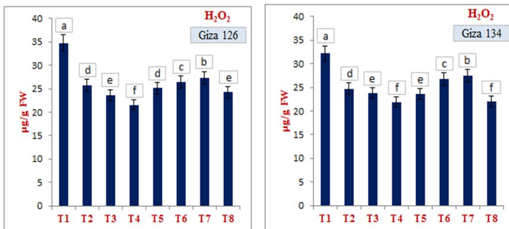
Figure (2): Effect of SA and Chitosan on down-regulation of H 2 O 2 concentration in the two studied barley genotypes, Giza 126 and Giza 134 under water stress conditions. T 1 =Control, T 2 =100ppm, T 3 =200ppm, T 4 =300ppm of salicylic acid, T 5 =150ppm, T 6 =225ppm, T 7 =300ppm of chitosan and T 8 =salicylic acid 100ppm and chitosan 150ppm mixture.
