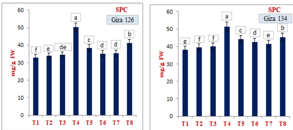
Figure (5): Effect of SA and Chitosan on total soluble protein content (SPC) in the two studied barley genotypes, Giza 126 and Giza 134 under water stress conditions.T 1 =Control, T 2 =100ppm, T 3 =200ppm, T 4 =300ppm of salicylic acid, T 5 =150ppm, T 6 =225ppm, T 7 =300ppm of chitosan and T 8 =salicylic acid 100ppm and chitosan 150ppm mixture.
