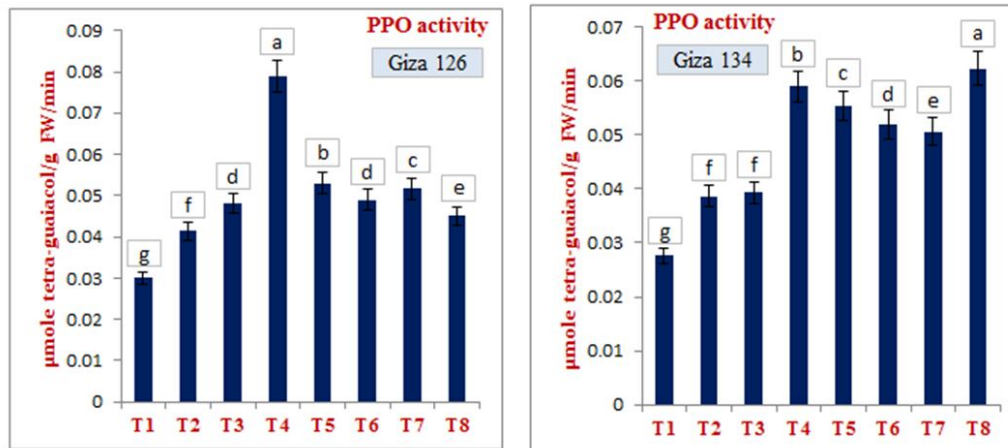
Figure (9): Effect of Salicylic Acid (SA) and Chitosan on polyphenol oxidase (PPO) activity in barley leaves for the two studied genotypes, Giza 126 and Giza 134 under water stress conditions. T 1 =Control, T 2 =100ppm, T 3 =200ppm, T 4 =300ppm of salicylic acid, T 5 =150ppm, T 6 =225ppm, T 7 =300ppm of chitosan and T 8 =salicylic acid 100ppm and chitosan 150ppm mixture.
