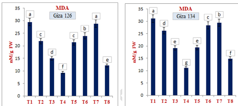
Figure (1): Effect of SA and Chitosan on down-regulation of malondialdehyde (MDA) level in the two studied barley genotypes, Giza 126 and Giza 134 under water stress conditions. T 1 =Control, T 2 =100ppm, T 3 =200ppm, T 4 =300ppm of salicylic acid, T 5 =150ppm, T 6 =225ppm, T 7 =300ppm of chitosan and T 8 =salicylic acid 100ppm and chitosan 150ppm mixture.
