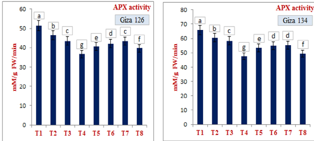
Figure (8): Effect of Salicylic Acid (SA) and Chitosan on Ascorbic peroxidase (APX) activity in barley leaves for the two studied genotypes, Giza 126 and Giza 134 under water stress conditions. T 1 =Control, T 2 =100ppm, T 3 =200ppm, T 4 =300ppm of salicylic acid, T 5 =150ppm, T 6 =225ppm, T 7 =300ppm of chitosan and T 8 =salicylic acid 100ppm and chitosan 150ppm mixture.
