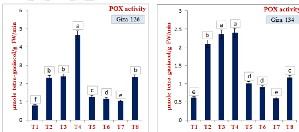
Figure (7): Effect of Salicylic Acid (SA) and Chitosan on Peroxidase (POX) activity in barley leaves for the two studied genotypes, Giza 126 and Giza 134 under water stress conditions. T 1 =Control,
