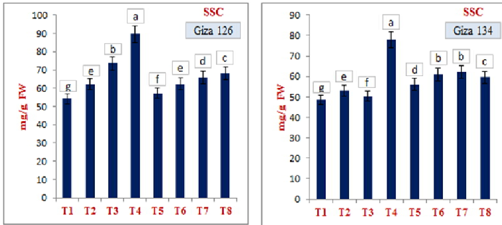
Figure(4):Effect of SA and chitosan on the soluble sugars content (SSC) in the two studied barley genotypes, Giza 126 and Giza 134 under water stress conditions.T 1 =Control, T 2 =100ppm, T 3 =200ppm, T 4 =300ppm of salicylic acid, T 5 =150ppm, T 6 =225ppm, T 7 =300ppm of chitosan and T 8 =salicylic acid 100ppm and chitosan 150ppm mixture.
