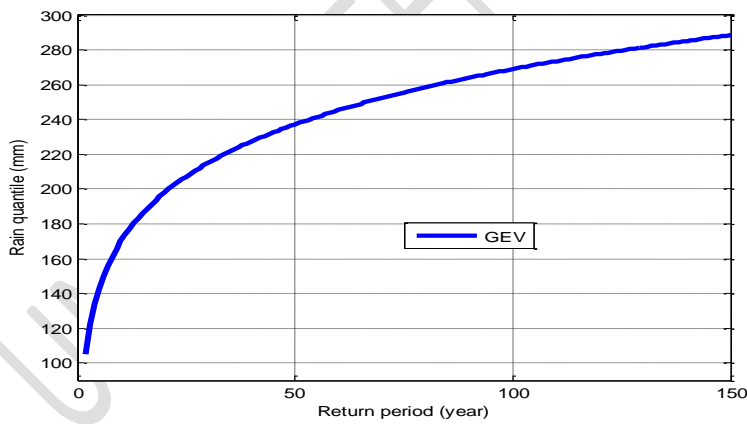
Figure 3: Quantile of rain in Cotonou according to the return periods.
