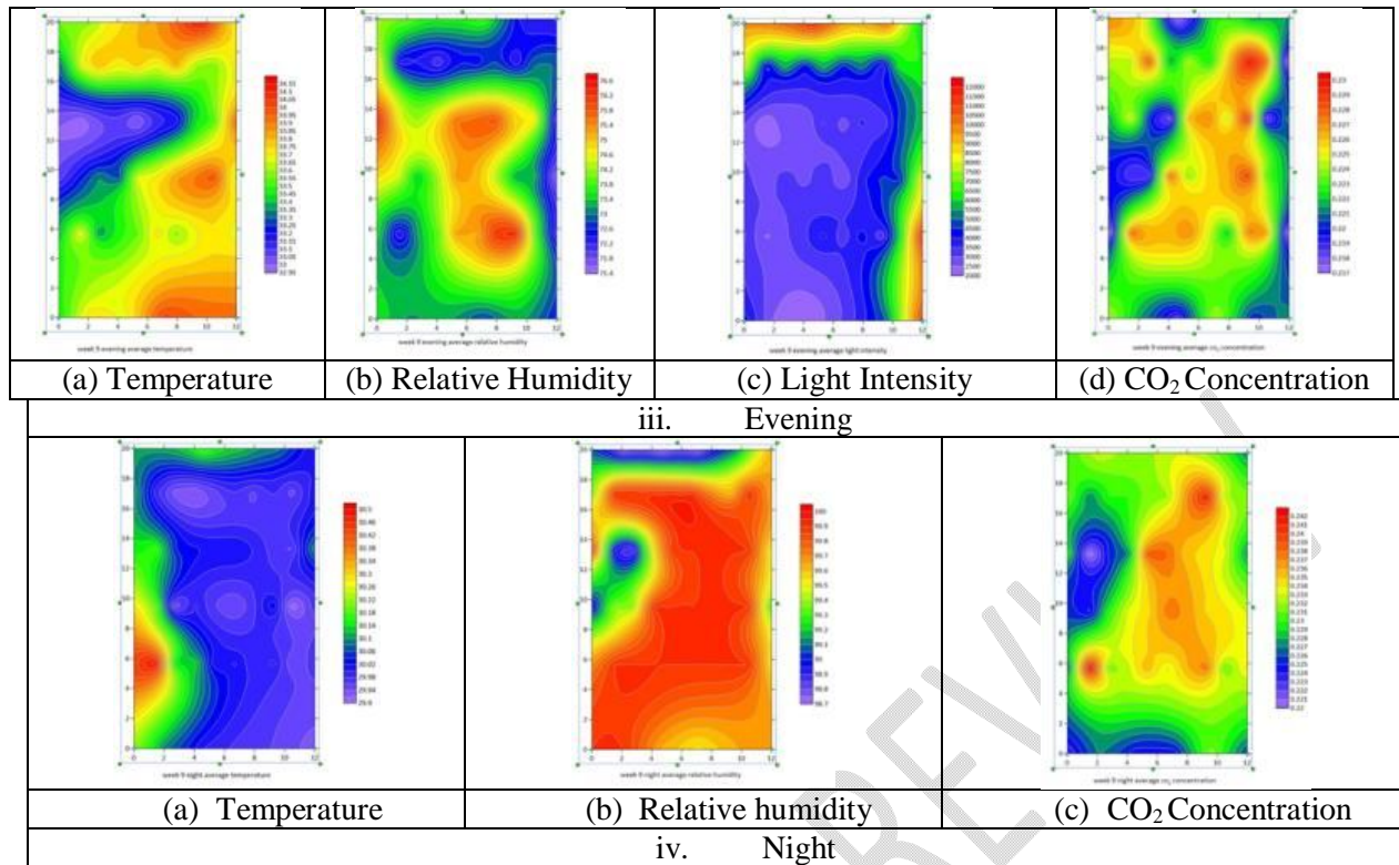
Figure 11 Spatial variation of microclimate in week 9 inside the polyhouse
