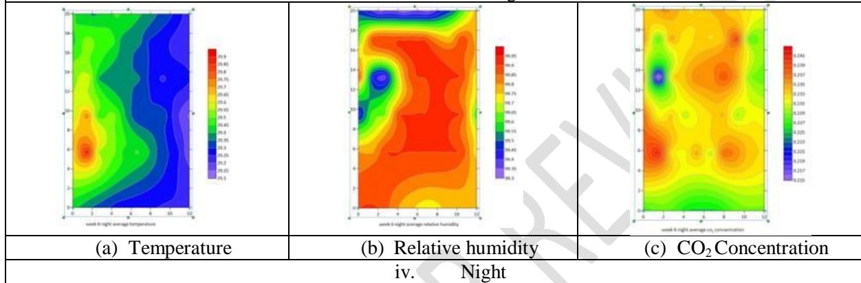
Figure 8 Spatial variation of microclimate in week 6 inside the polyhouse
