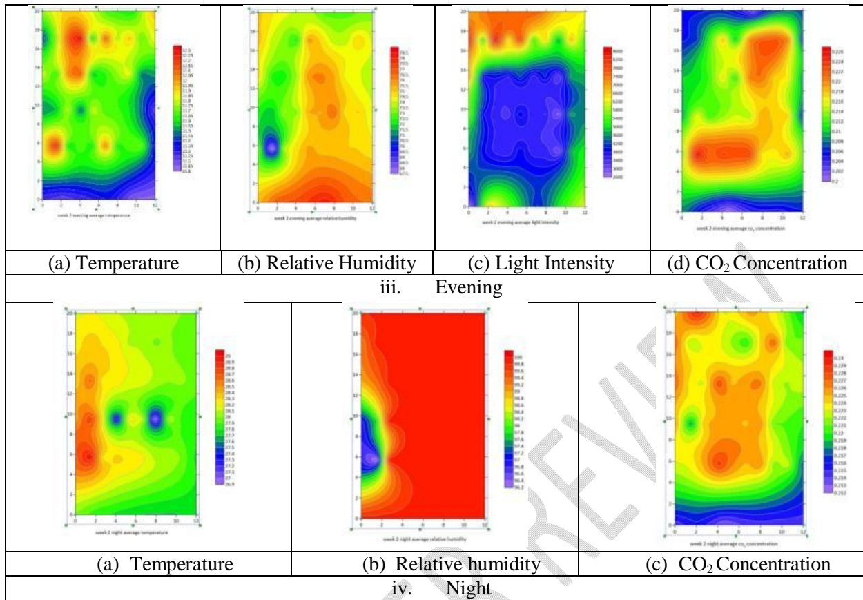
Figure 4 Spatial variation of microclimate in week 2 inside the polyhouse
