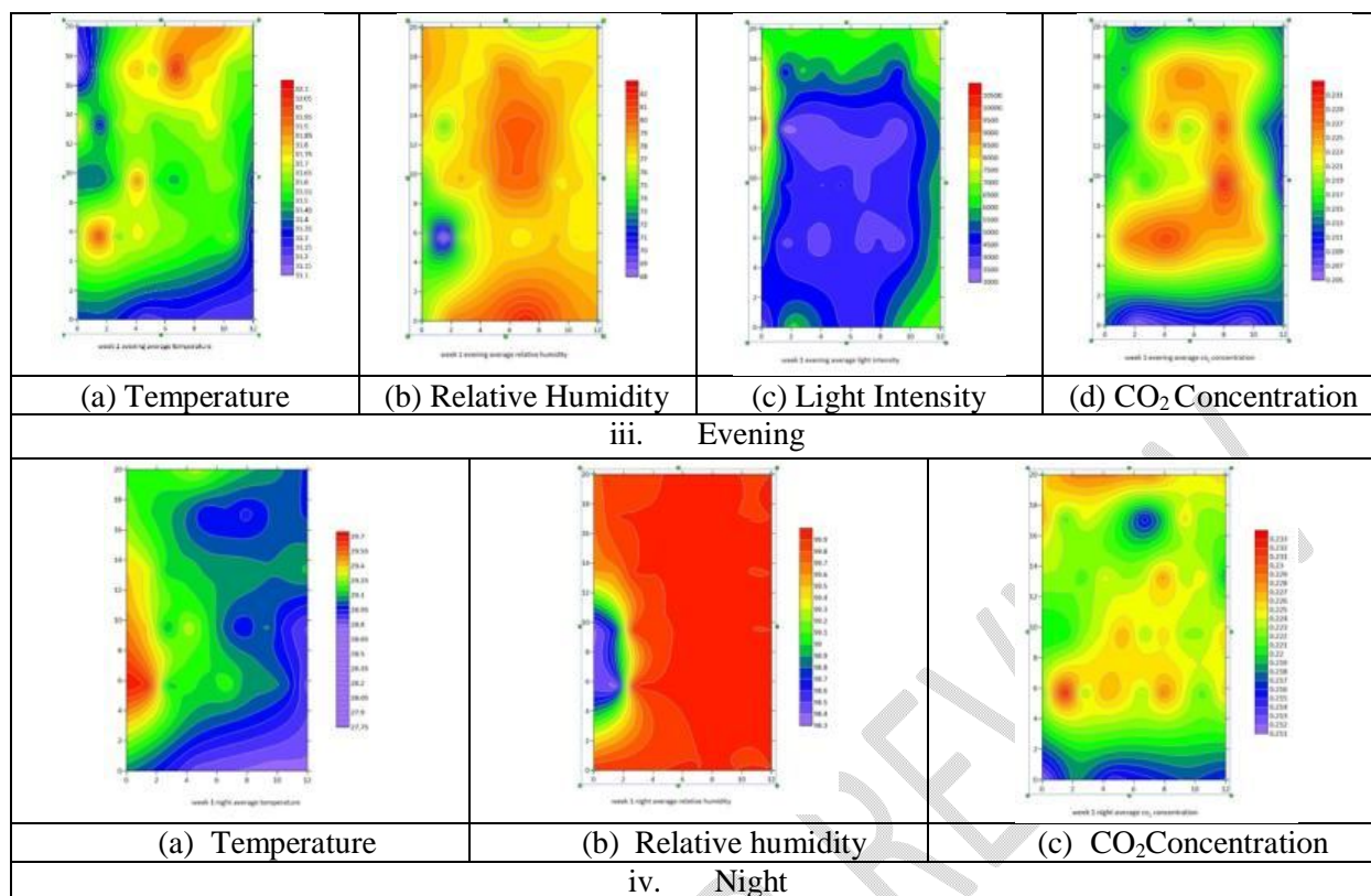
Figure 3 Spatial variation of microclimate in week 1 inside the polyhouse
