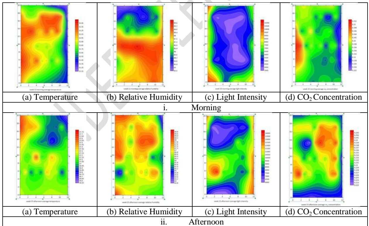
Figure 14 Spatial variation of microclimate in week 12 inside the polyhouse
