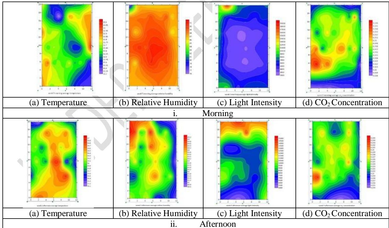
Figure 6 Spatial variation of microclimate in week 4 inside the polyhouse
