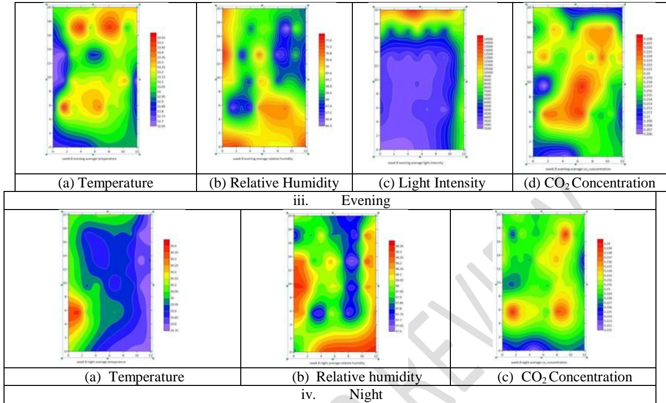
Figure 10 Spatial variation of microclimate in week 8 inside the polyhouse
