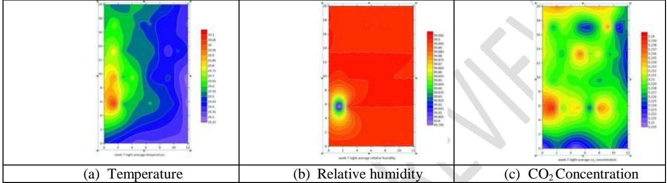
Figure 9 Spatial variation of microclimate in week 7 inside the polyhouse
