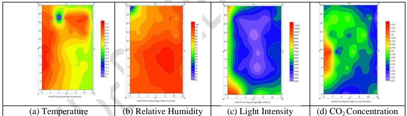
Figure 9 Spatial variation of microclimate in week 7 inside the polyhouse
