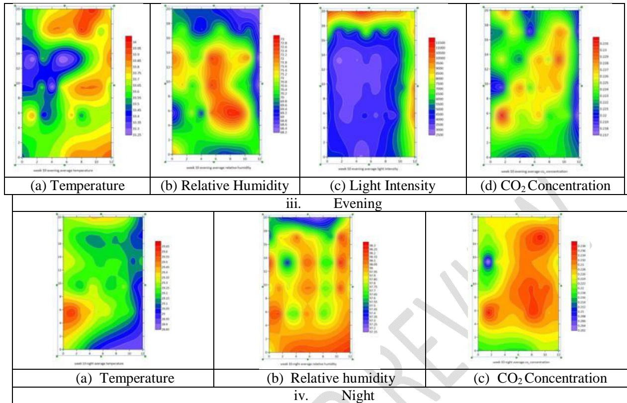
Figure 12 Spatial variation of microclimate in week 10 inside the polyhouse
