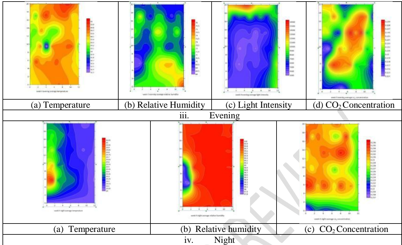
Figure 6 Spatial variation of microclimate in week 4 inside the polyhouse
