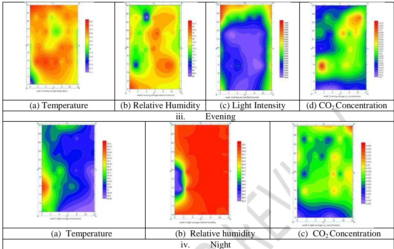
Figure 7 Spatial variation of microclimate in week 5 inside the polyhouse
