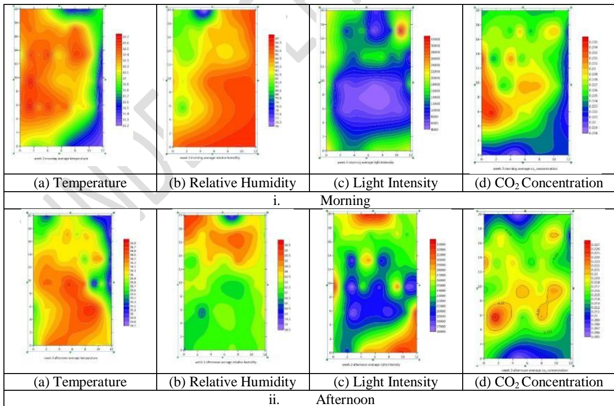
Figure 4 Spatial variation of microclimate in week 2 inside the polyhouse
