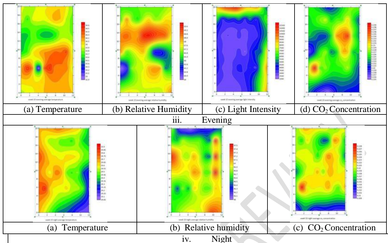
Figure 15 Spatial variation of microclimate in week 13 inside the polyhouse
