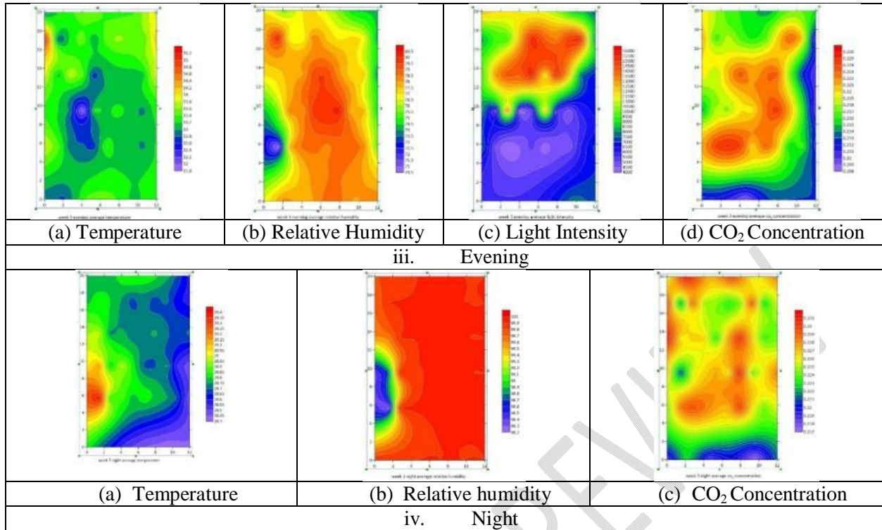
Figure 5 Spatial variation of microclimate in week 3 inside the polyhouse
