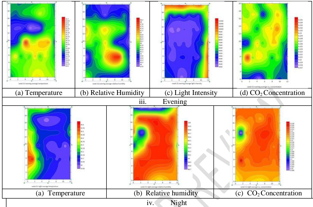
Figure 13 Spatial variation of microclimate in week 11 inside the polyhouse
