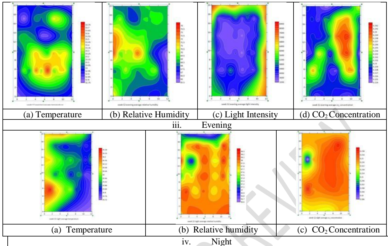
Figure 14 Spatial variation of microclimate in week 12 inside the polyhouse
