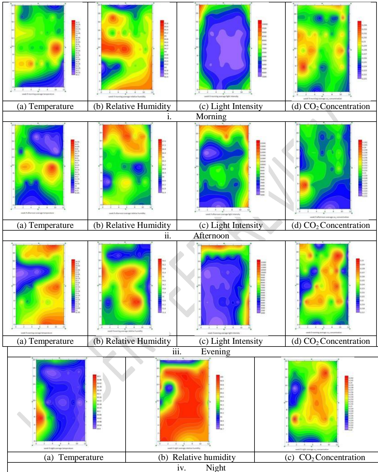
Figure 11 Spatial variation of microclimate in week 9 inside the polyhouse
