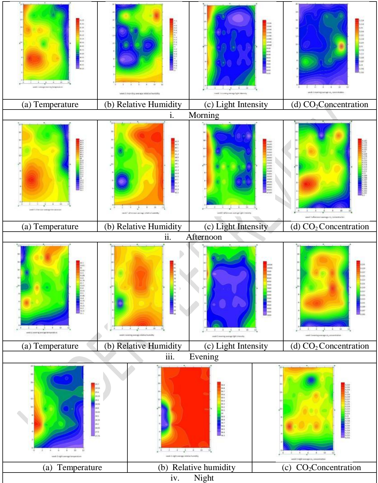
Figure 3 Spatial variation of microclimate in week 1 inside the polyhouse
