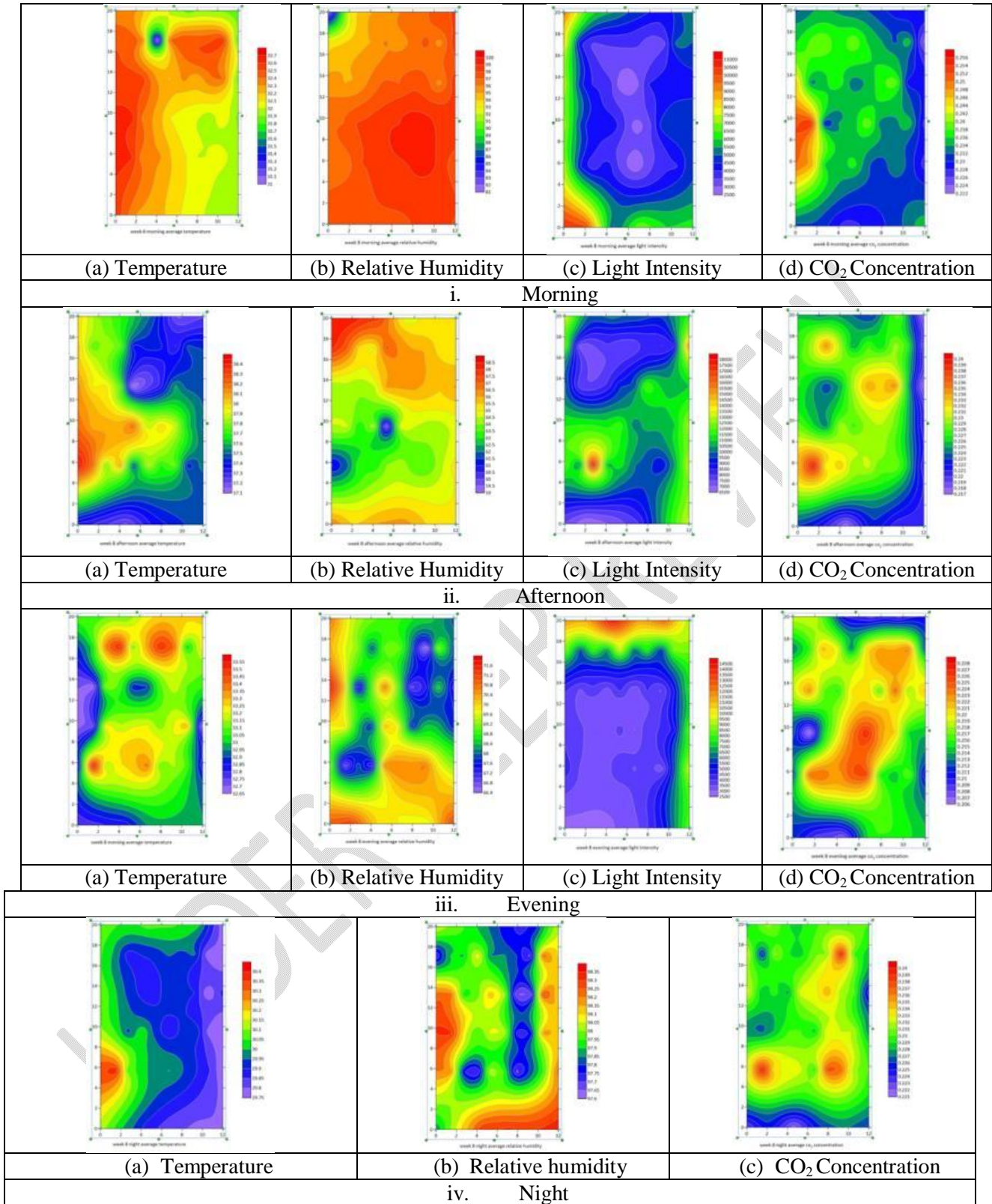
Figure 10 Spatial variation of microclimate in week 8 inside the polyhouse
