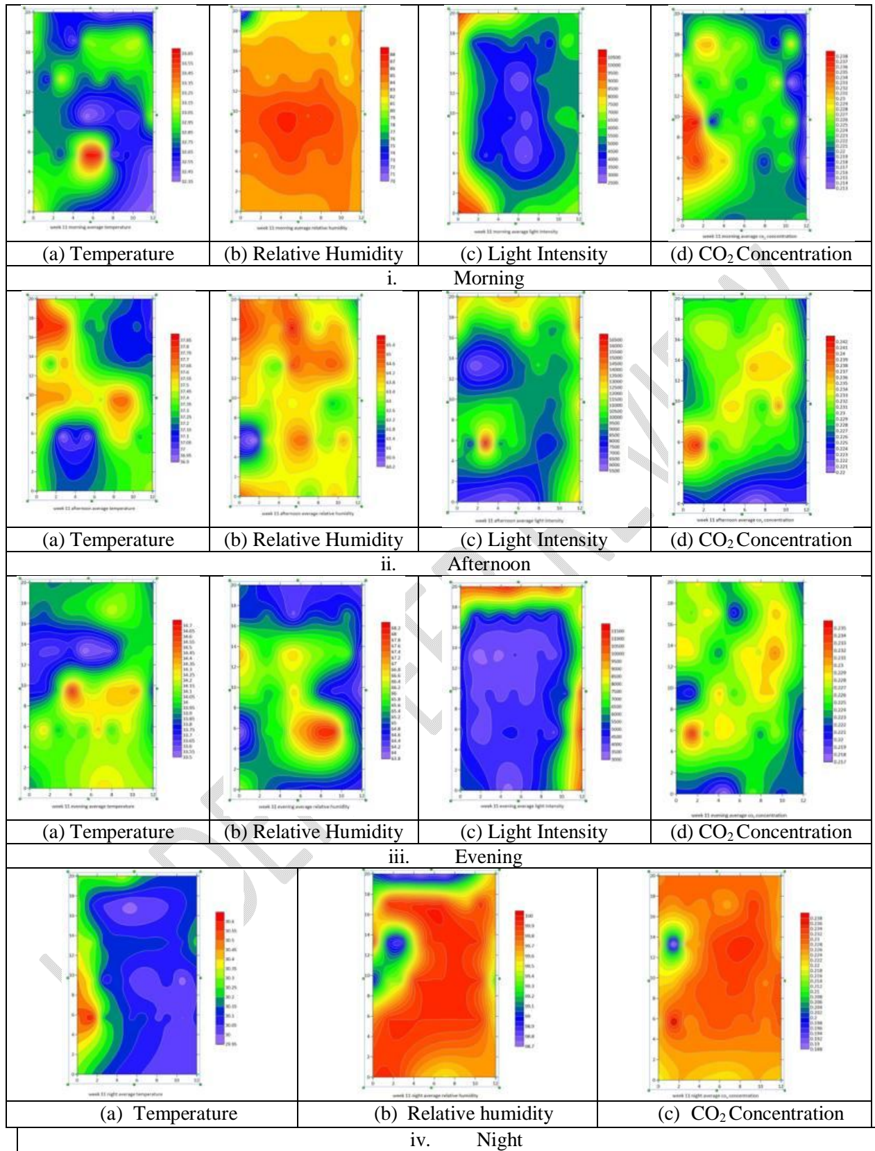
Figure 13 Spatial variation of microclimate in week 11 inside the polyhouse
