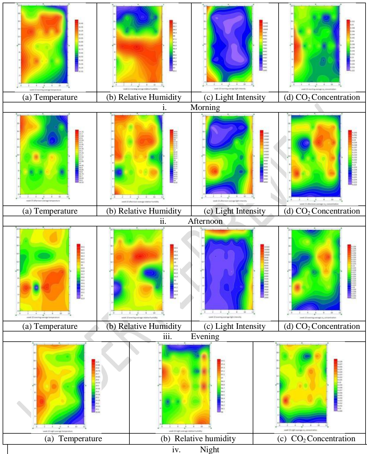
Figure 15 Spatial variation of microclimate in week 13 inside the polyhouse
