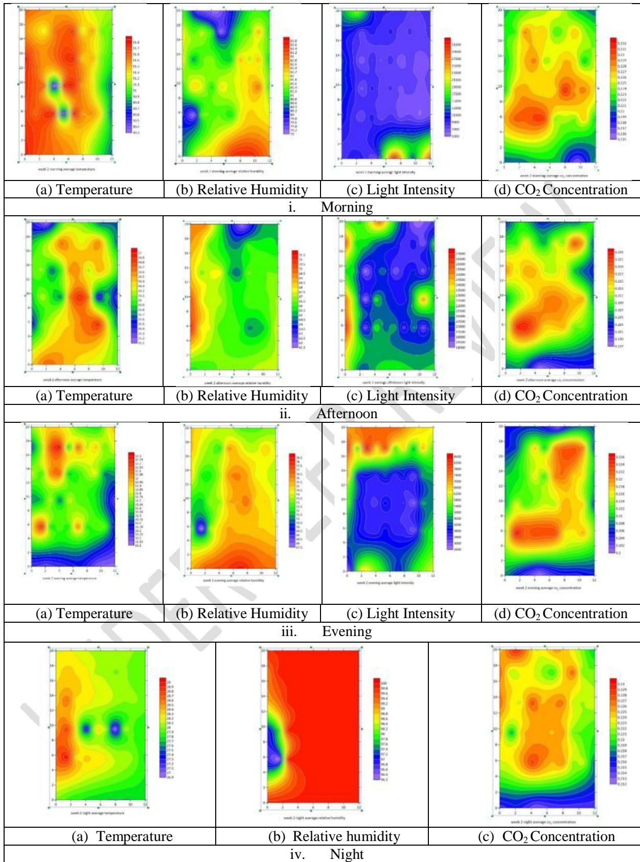
Figure 4 Spatial variation of microclimate in week 2 inside the polyhouse
