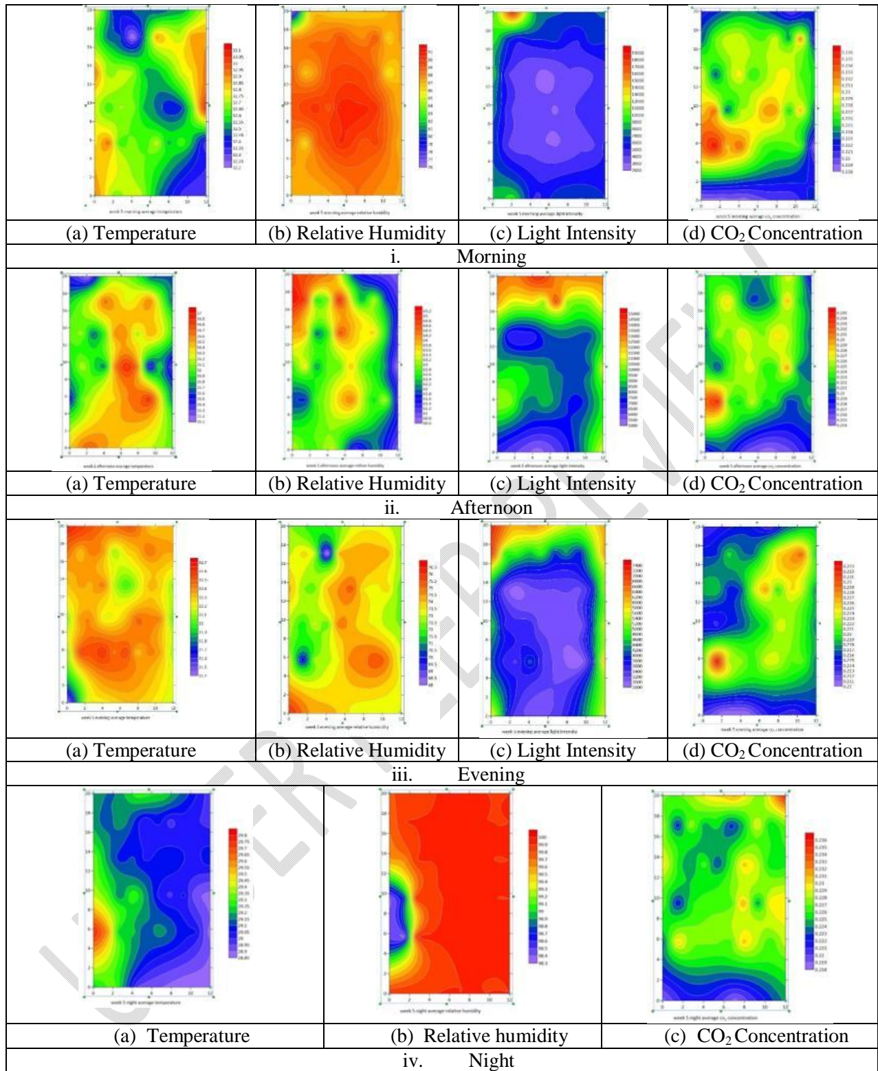
Figure 7 Spatial variation of microclimate in week 5 inside the polyhouse
