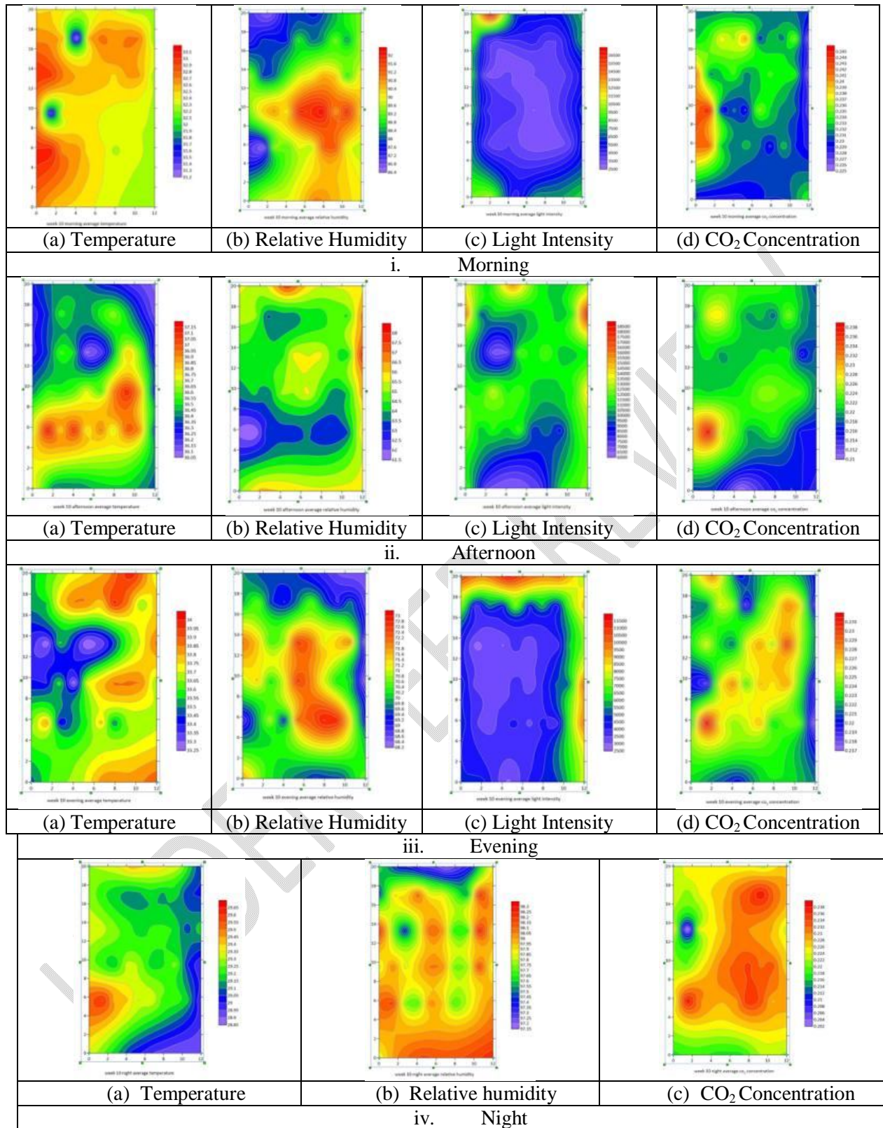
Figure 12 Spatial variation of microclimate in week 10 inside the polyhouse
