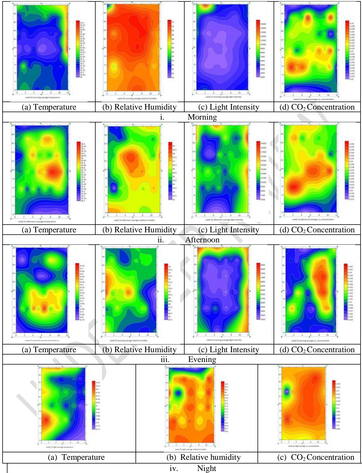
Figure 14 Spatial variation of microclimate in week 12 inside the polyhouse
