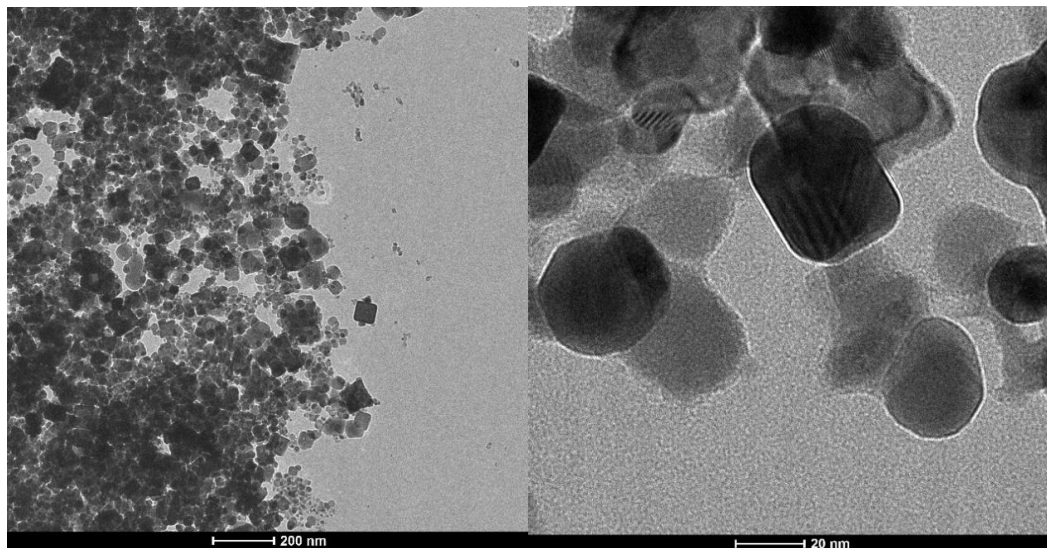
Figure 3 TEM images of C. Sativa mediated Cu_2O -ZnONPs nanoparticles
