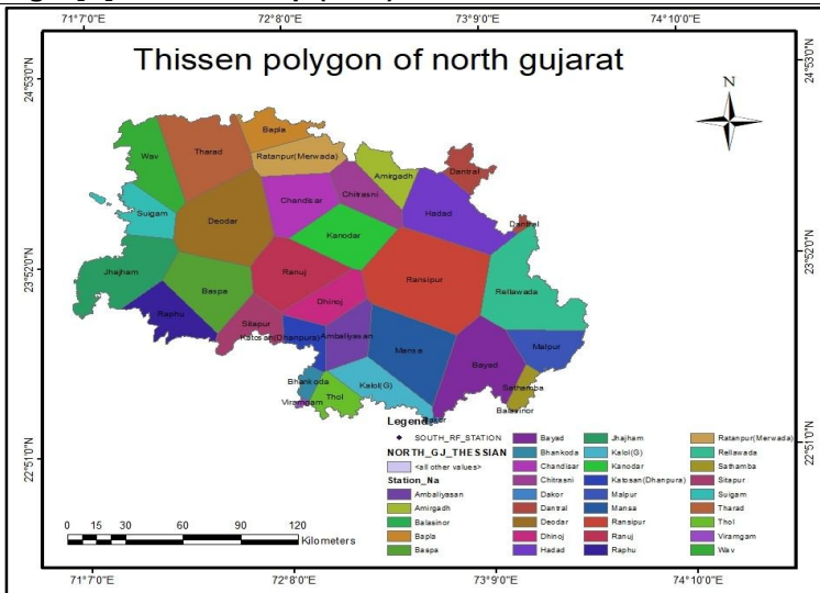
Fig. 3[C] Thiessen Polygon map for rain gauge stations
