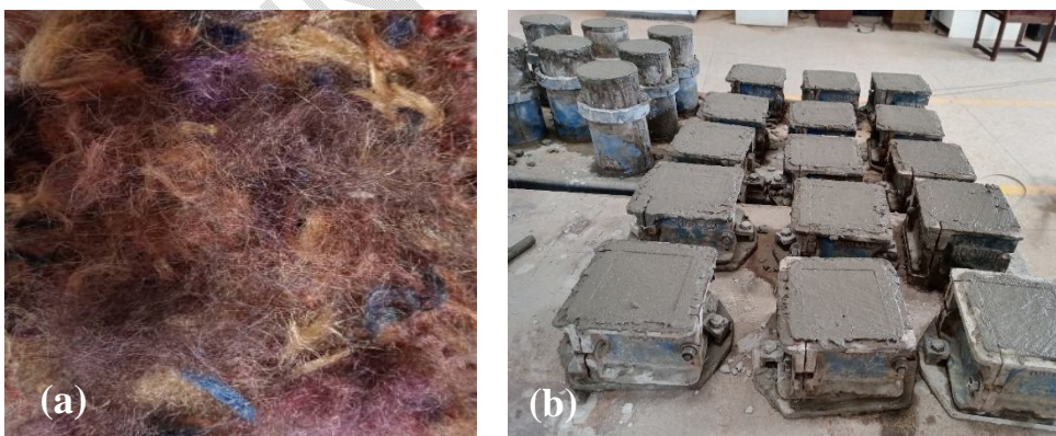
Figure 1: Material preparation: (a) waste synthetic hair fibre, (b) moulding of cube specimens
