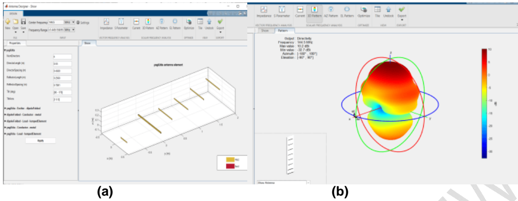
Fig. 12: MATLAB Antenna Designer Toolbox (a) Yagi Uda antenna (b) 3D radiation pattern
