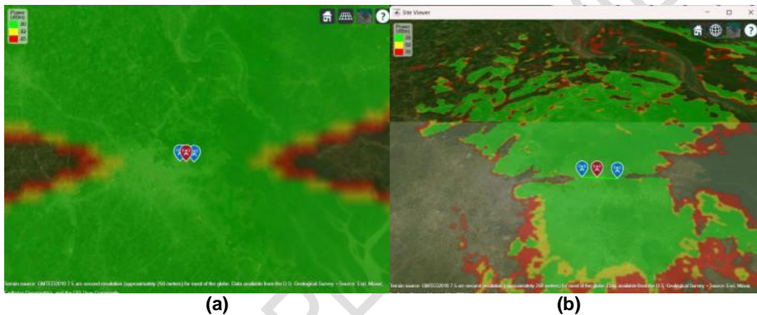
Fig. 13: Proposed campus radio coverage map using (a) Free Space model (b) Longley-Rice model
