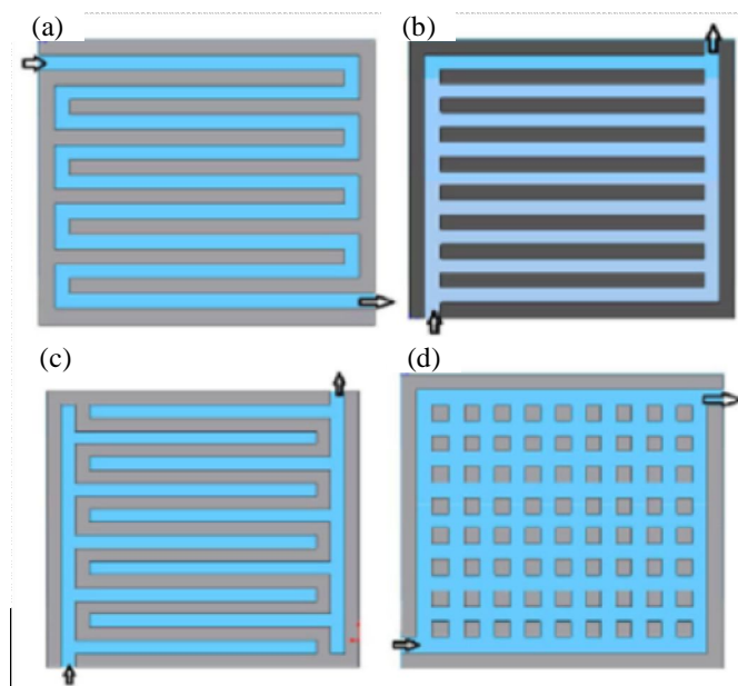
175 176 177 Fig.1 Schematic diagram of common flow field forms
