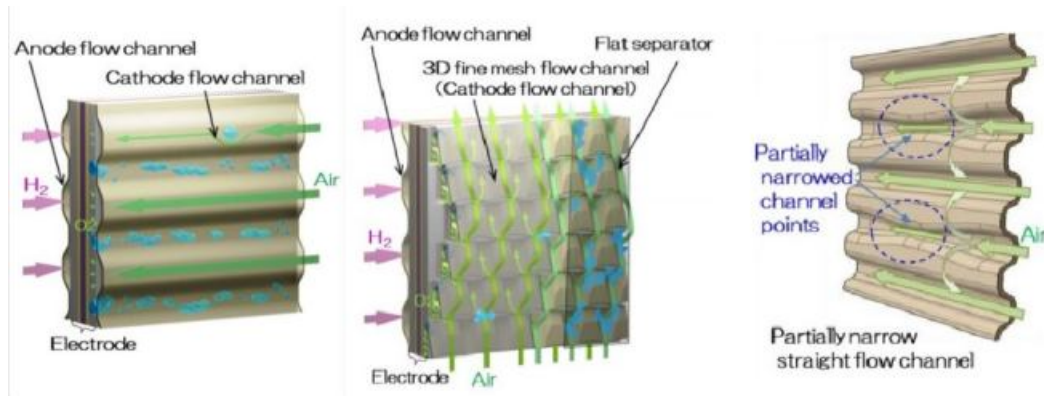
220 221 222 223 224 225 226 227 228 229 230 231 232 233 234 235 236 237 238 239 240 241 242 243 244 245 246 Figure 2 Flow field design of Toyota Mirai fuel cell
