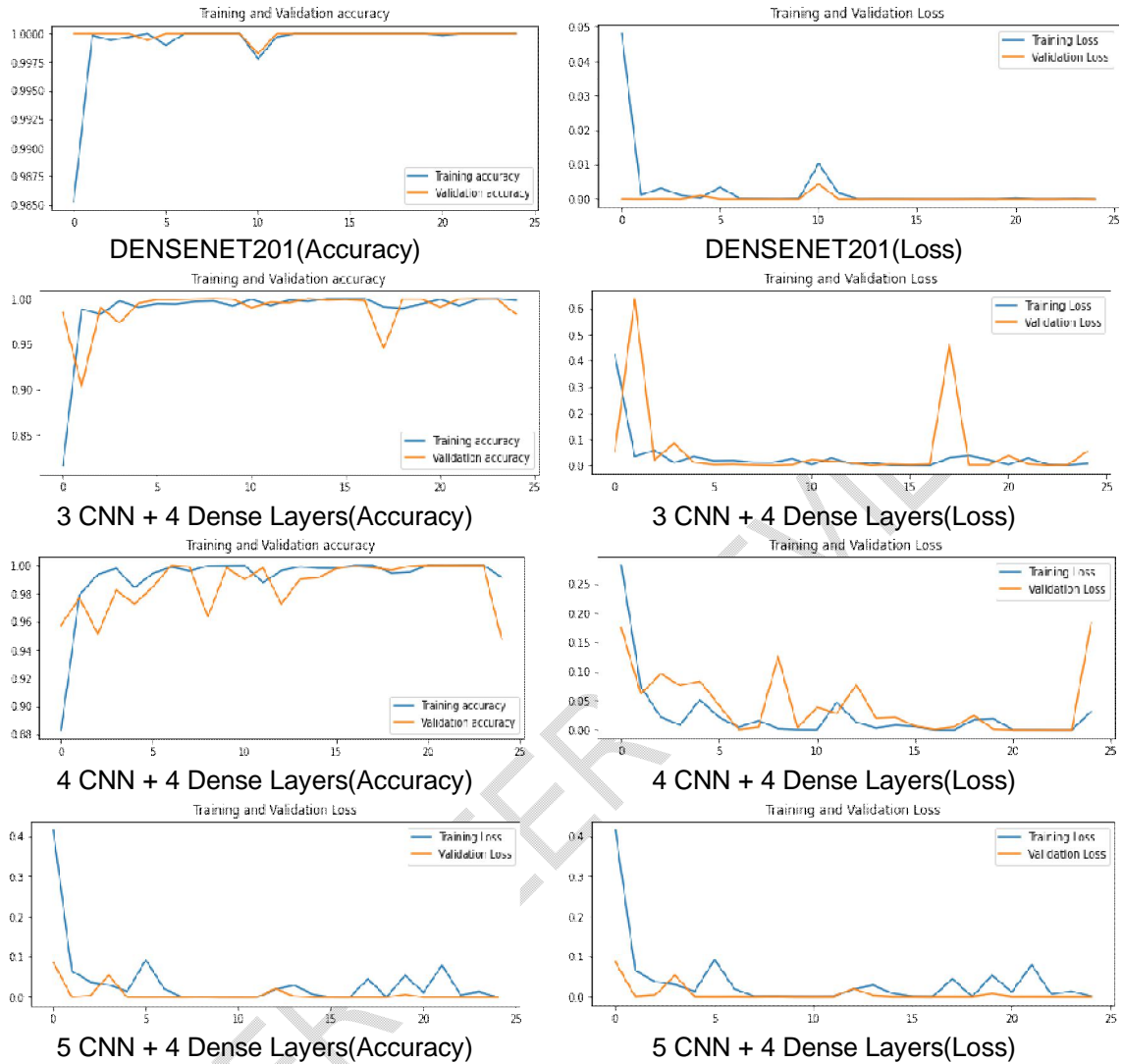
Figure 4. Accuracy – Loss Graph for Training and Validation Data Set
