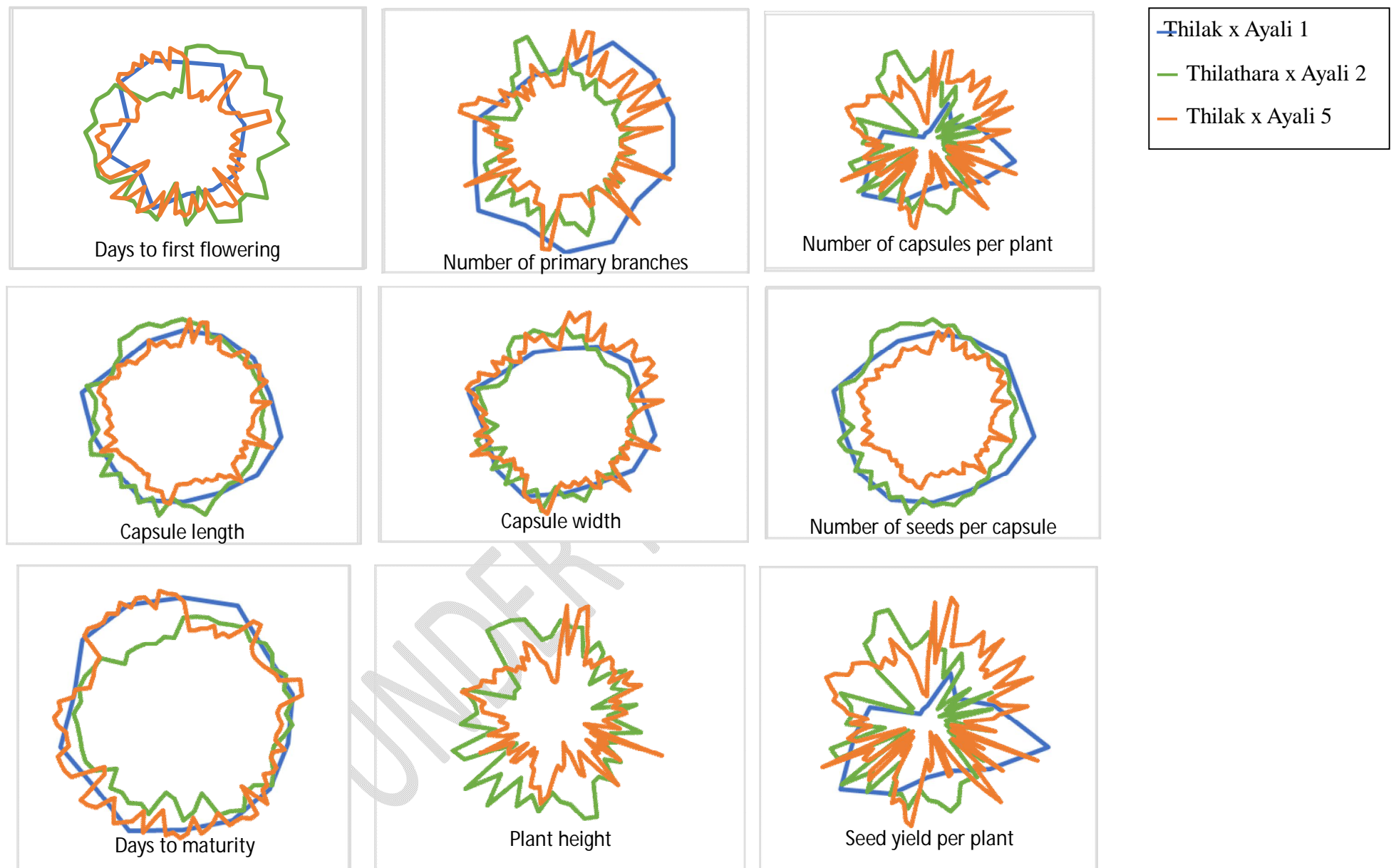
Fig 1. Variation for the yield related characters in the F 2 segregating populations of three crosses of sesame
